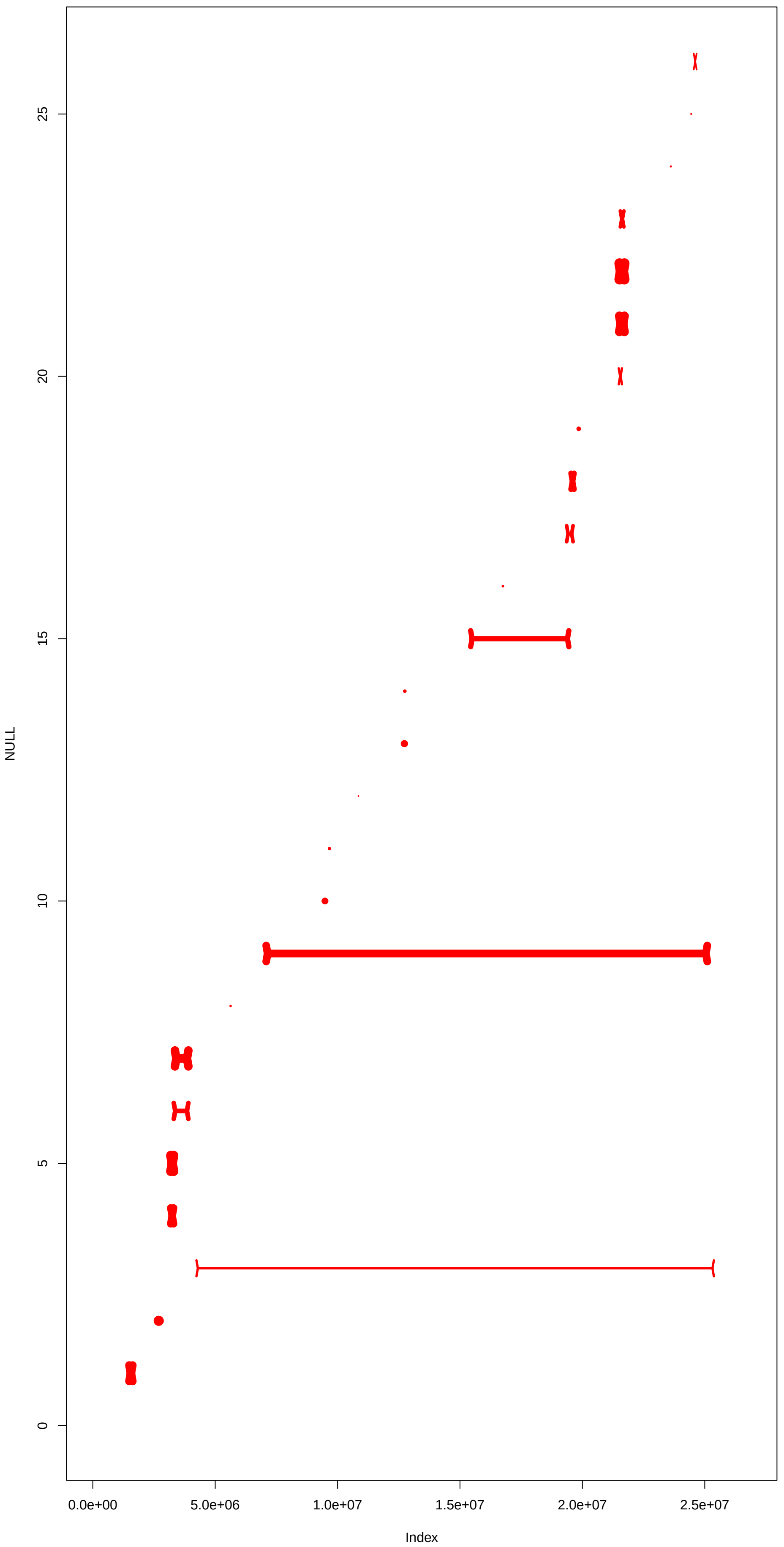
NC_044056.1 pass2
