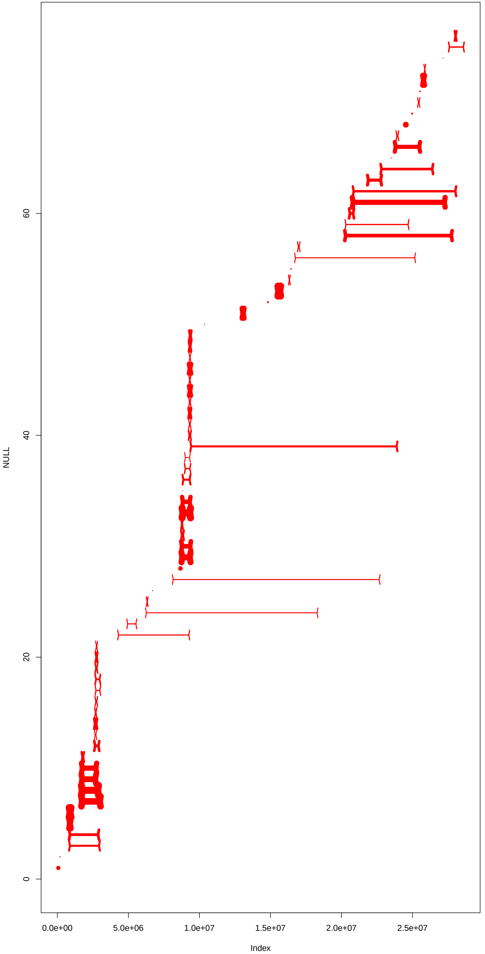
NC_044062.1 pass1
