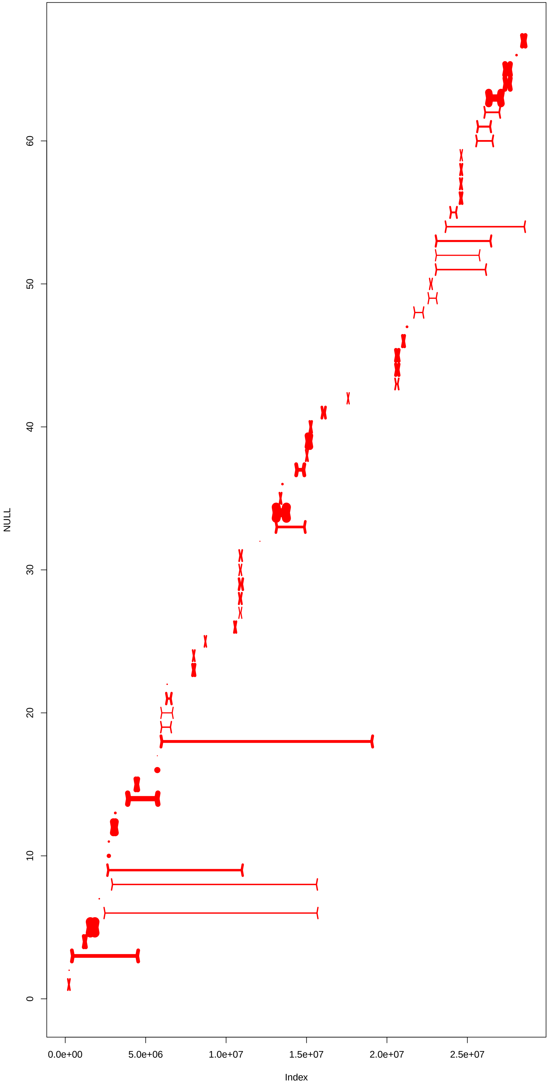
NC_044049.1 pass1
