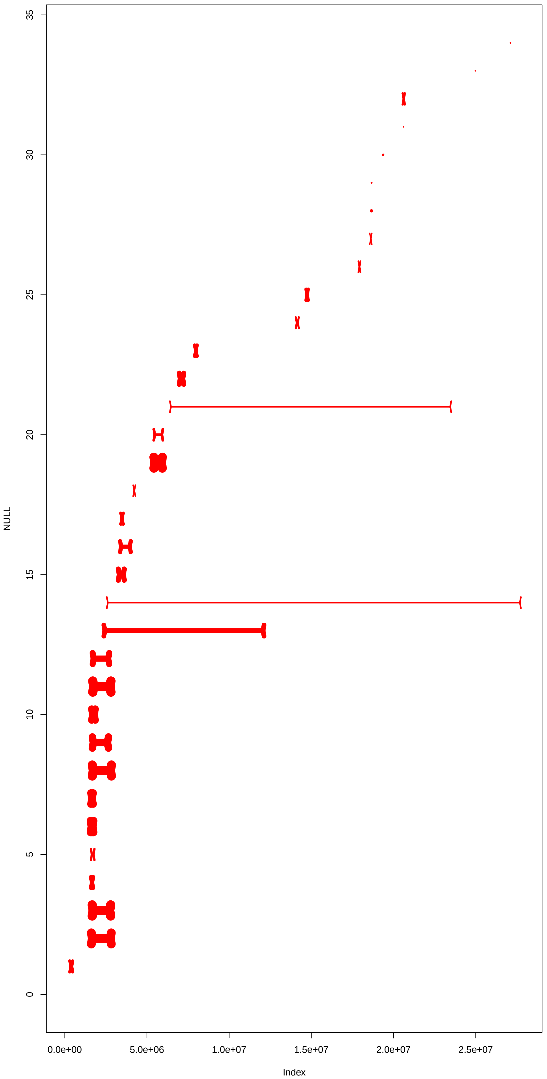
NC_044053.1 pass2
