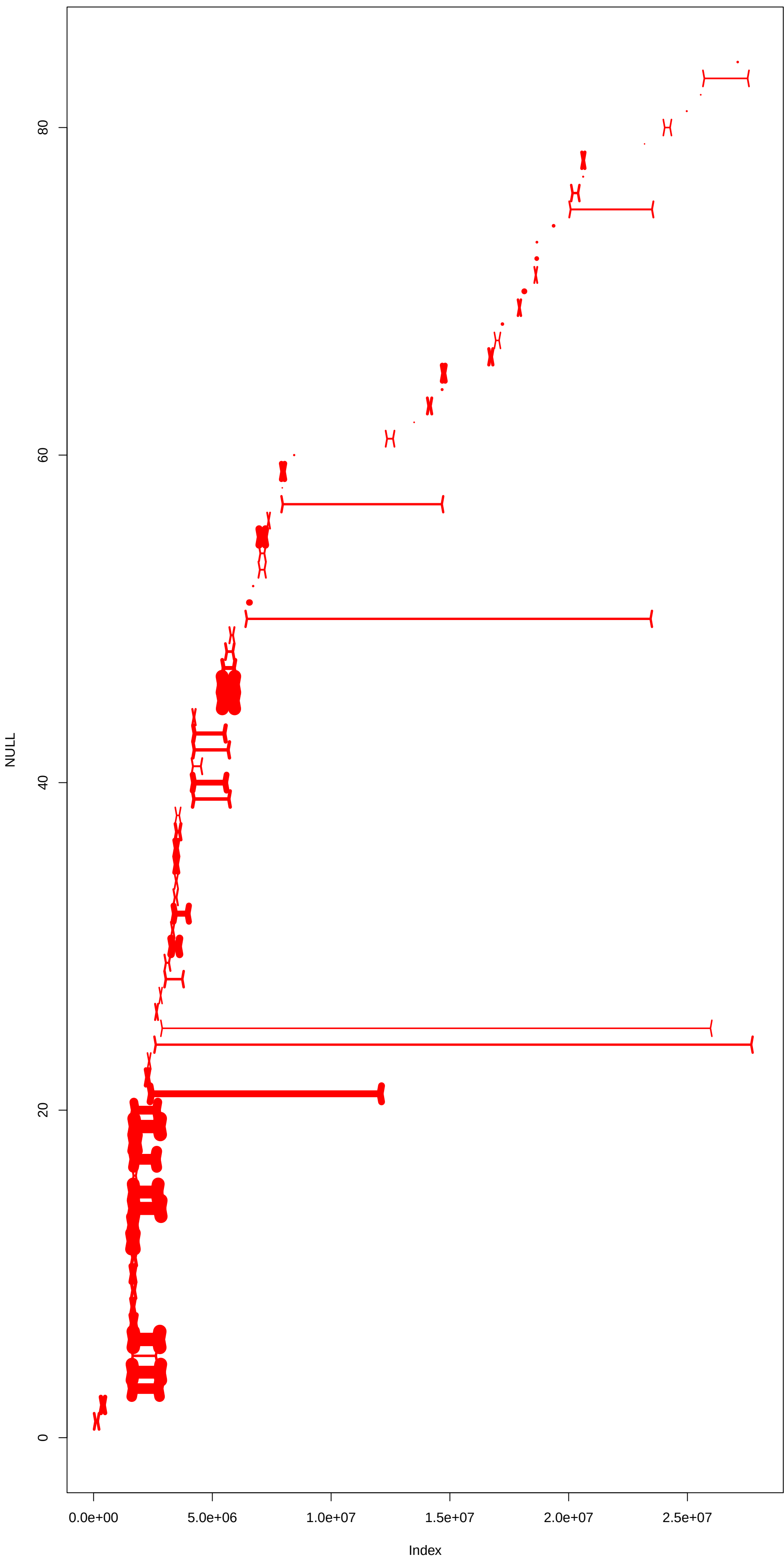
NC_044053.1 pass1
