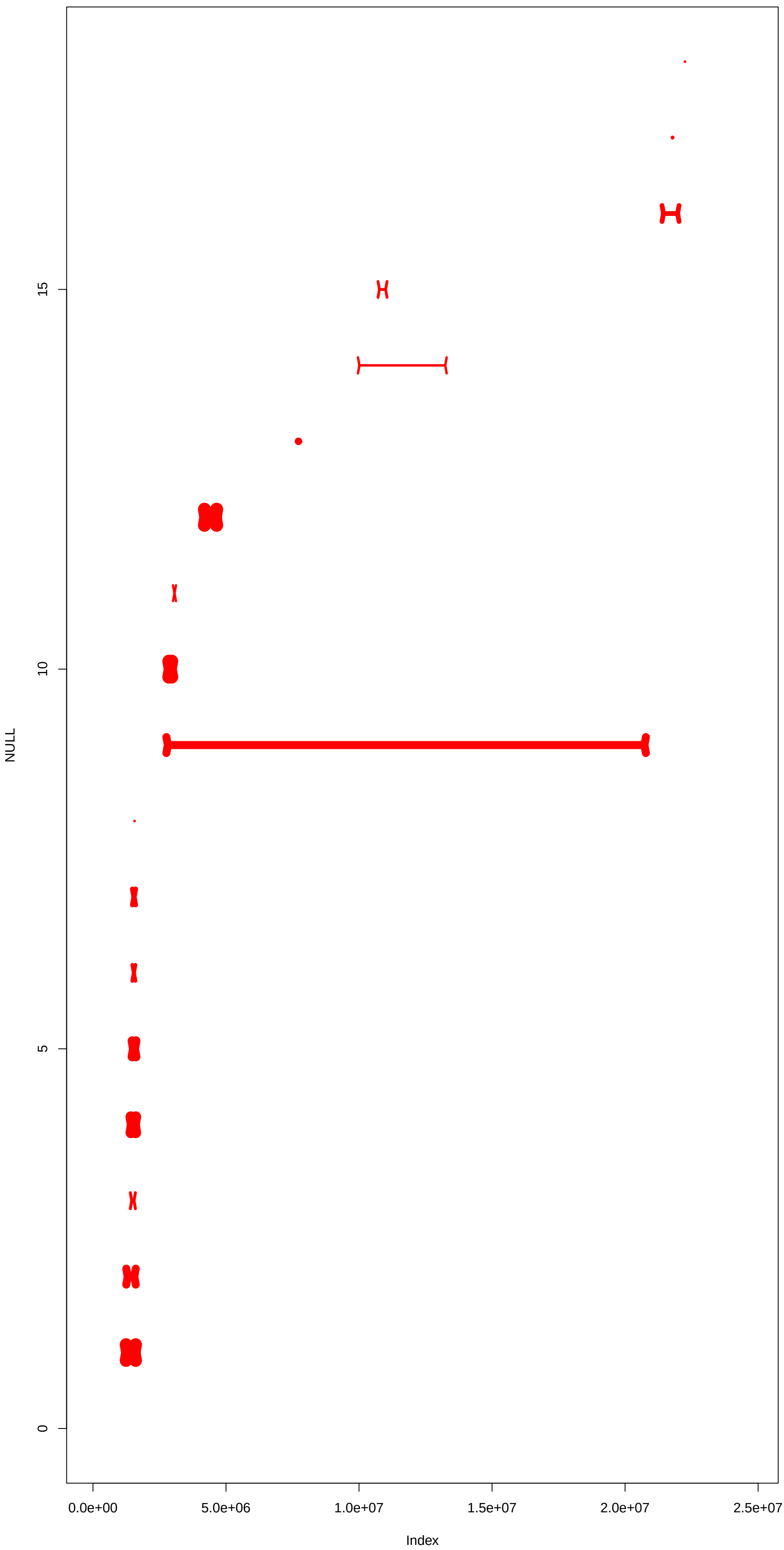
NC_044067.1 pass2
