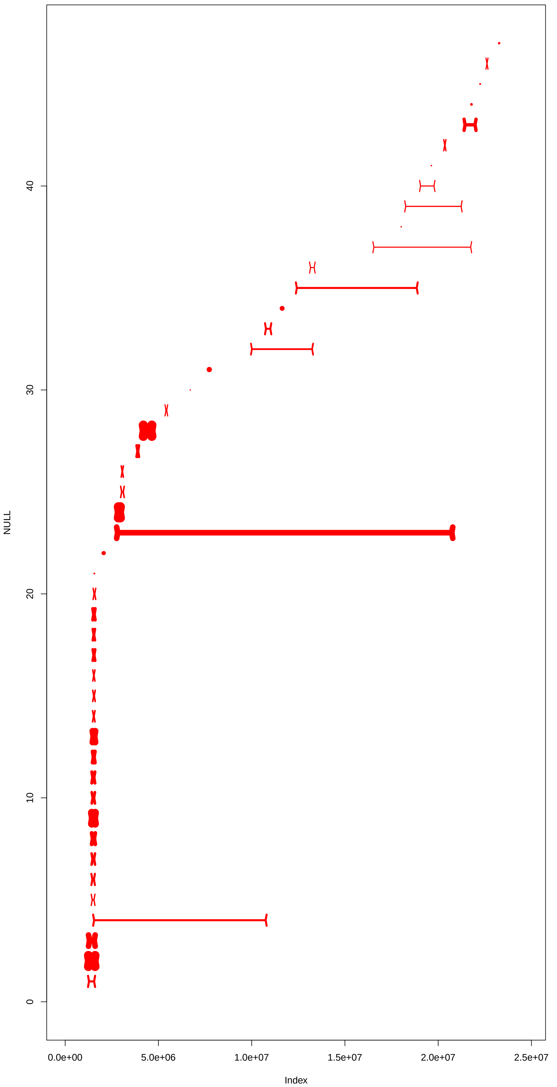
NC_044067.1 pass1
