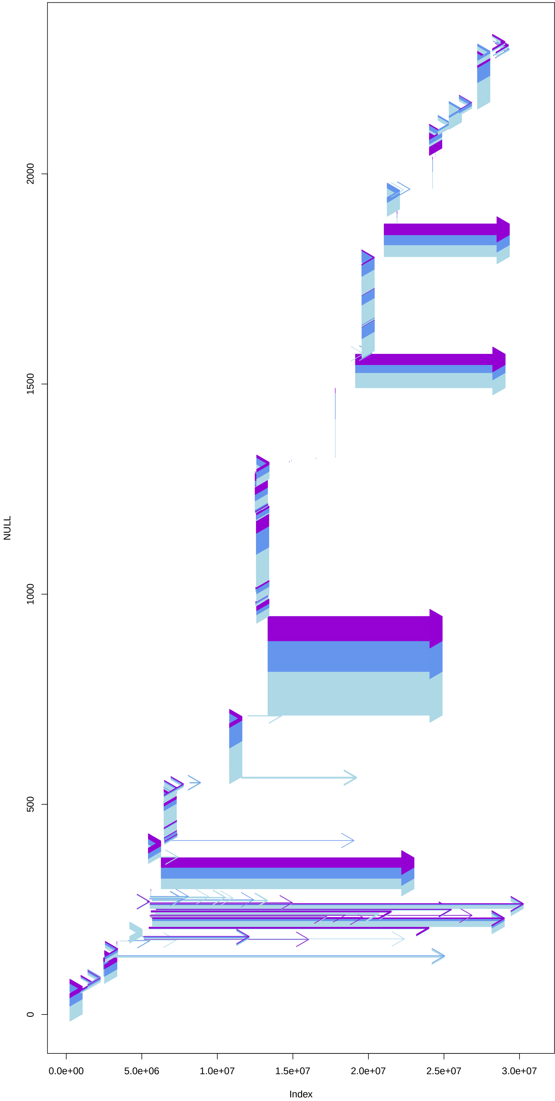
NC_044048.1 filtered 2 programs; 1 pass
