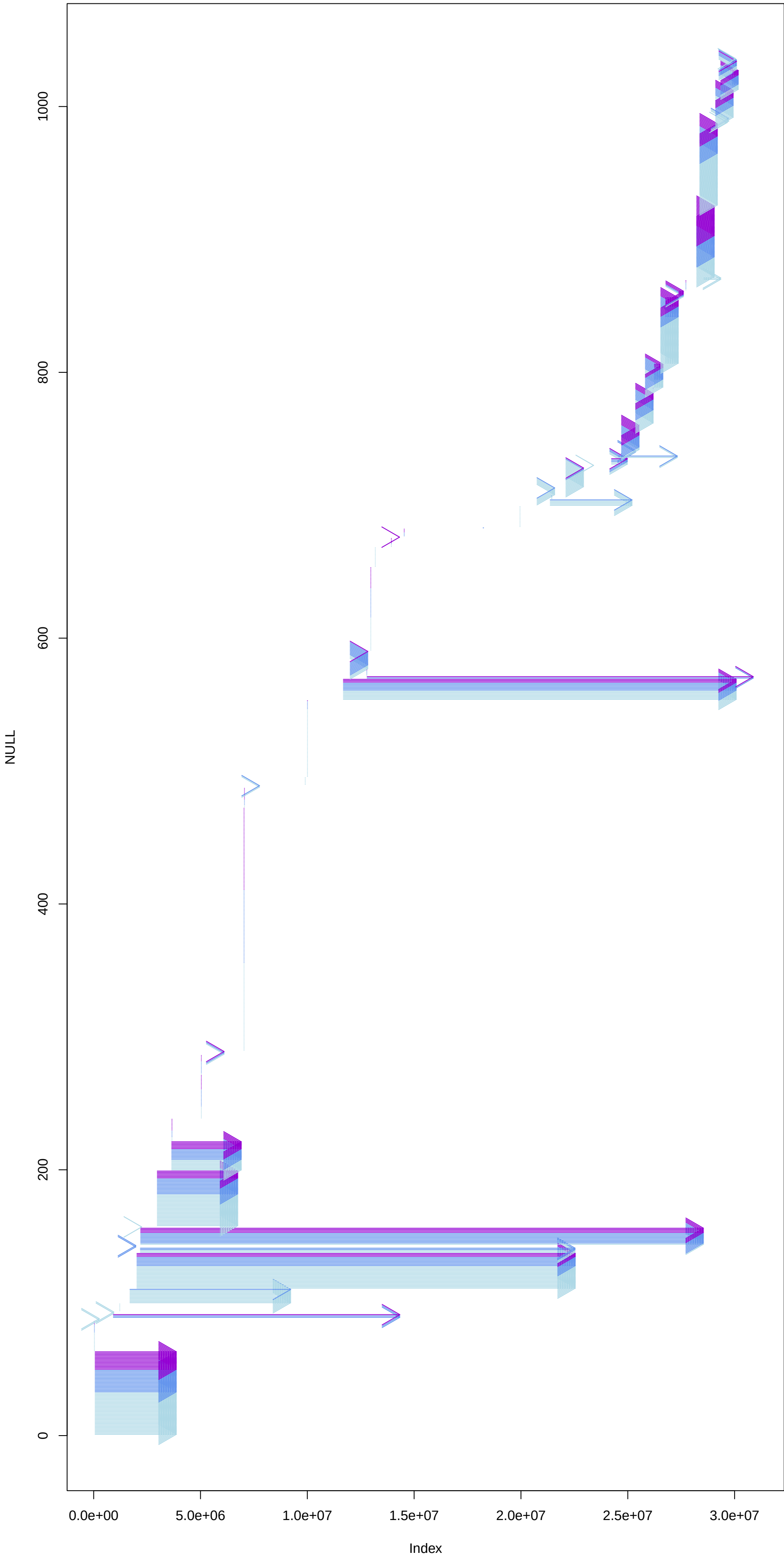
NC_044050.1 filtered 2 programs; 1 pass
