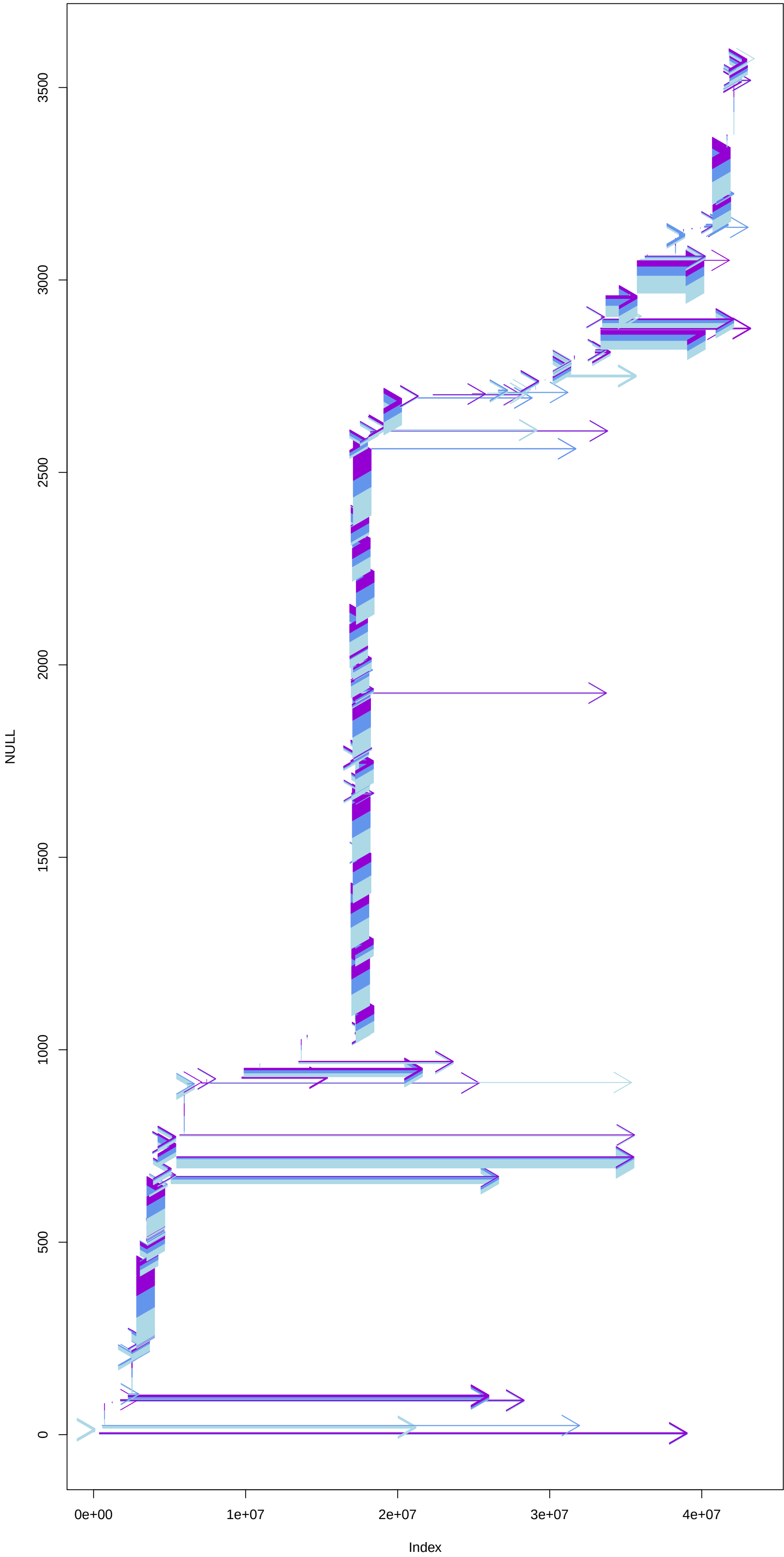
NC_044051.1 filtered 2 programs; 1 pass
