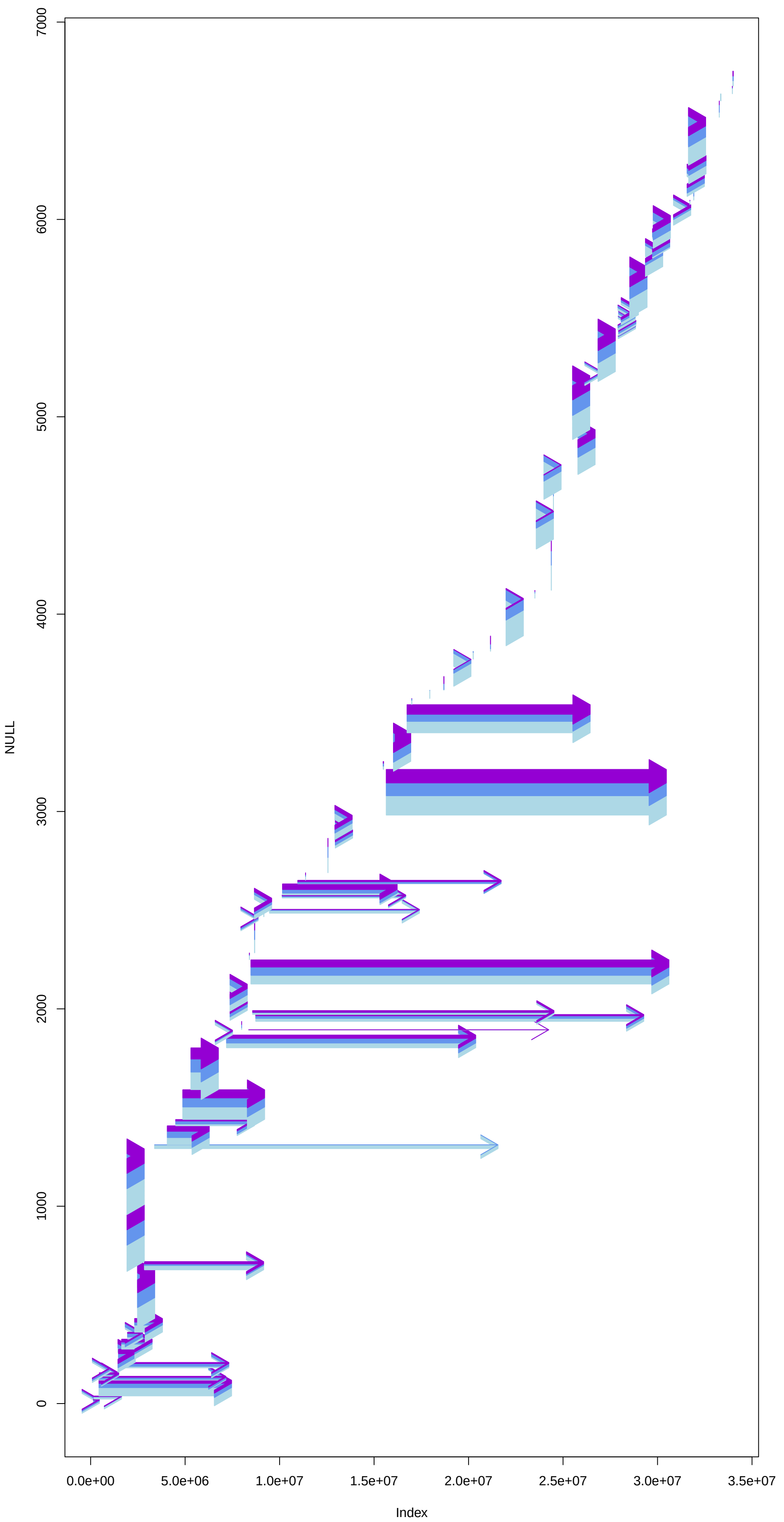
NC_044054.1
