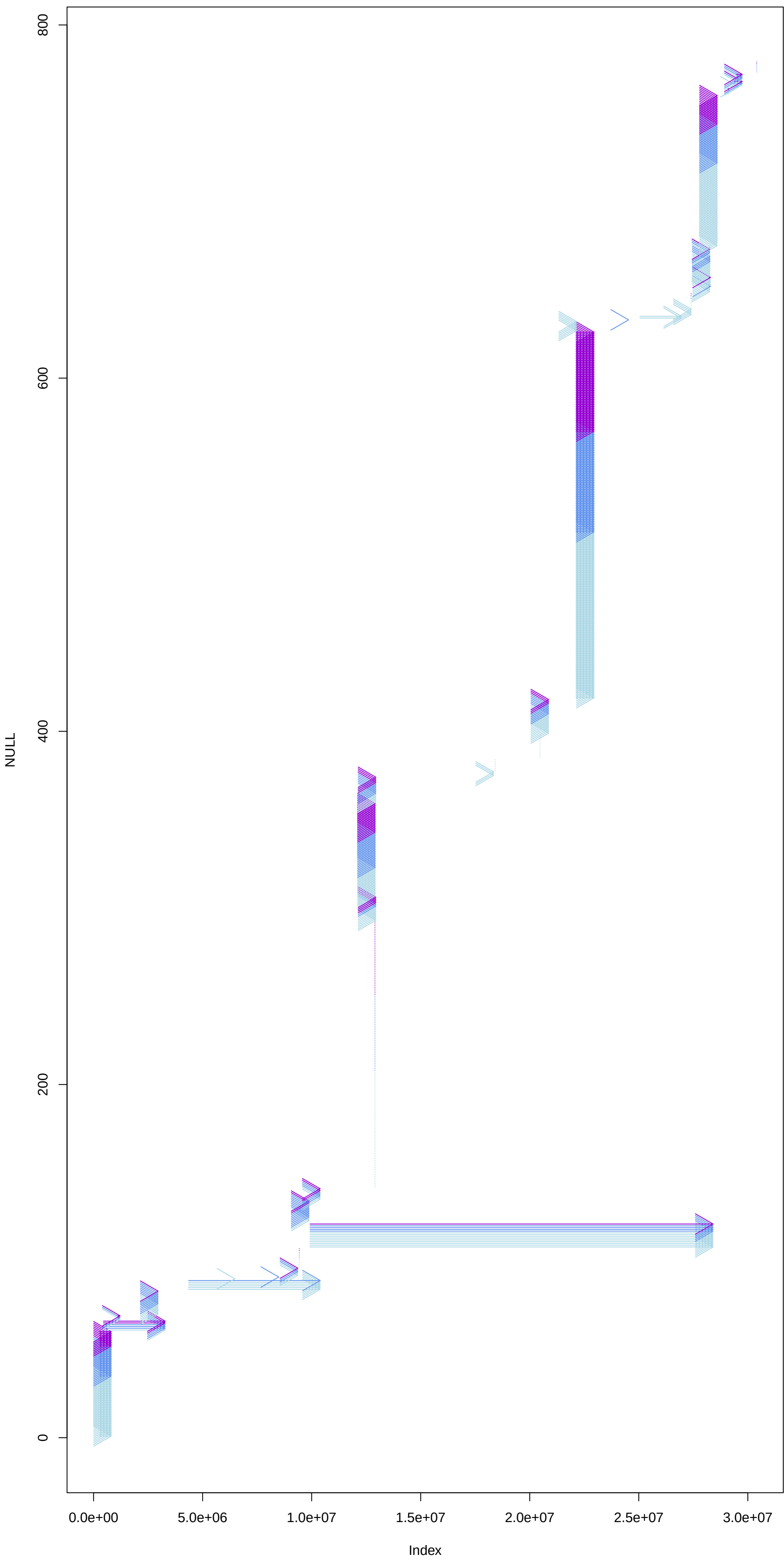
NC_044058.1 filtered 2 programs; 1 pass
