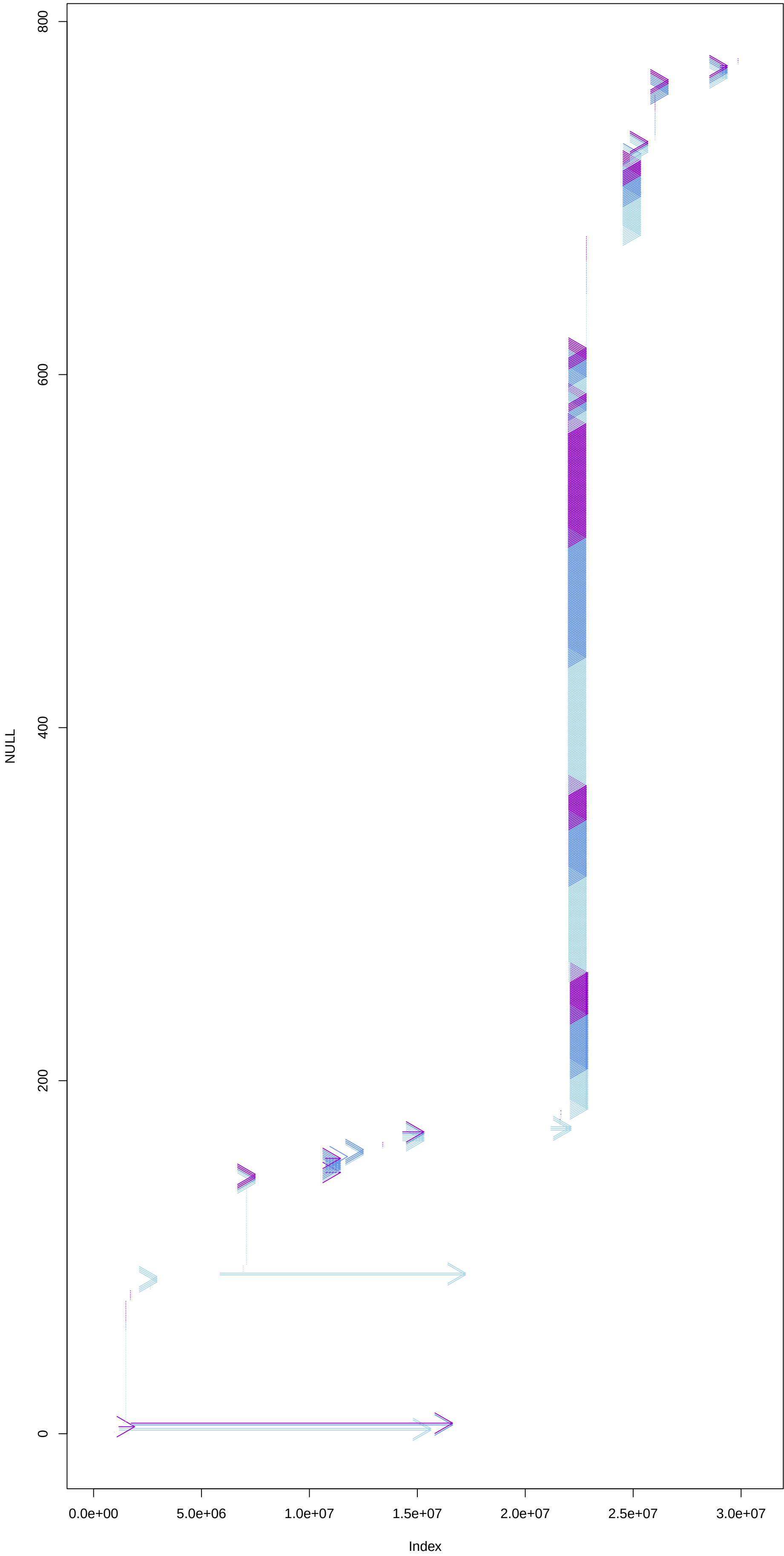
NC_044059.1 filtered 2 programs; 1 pass
