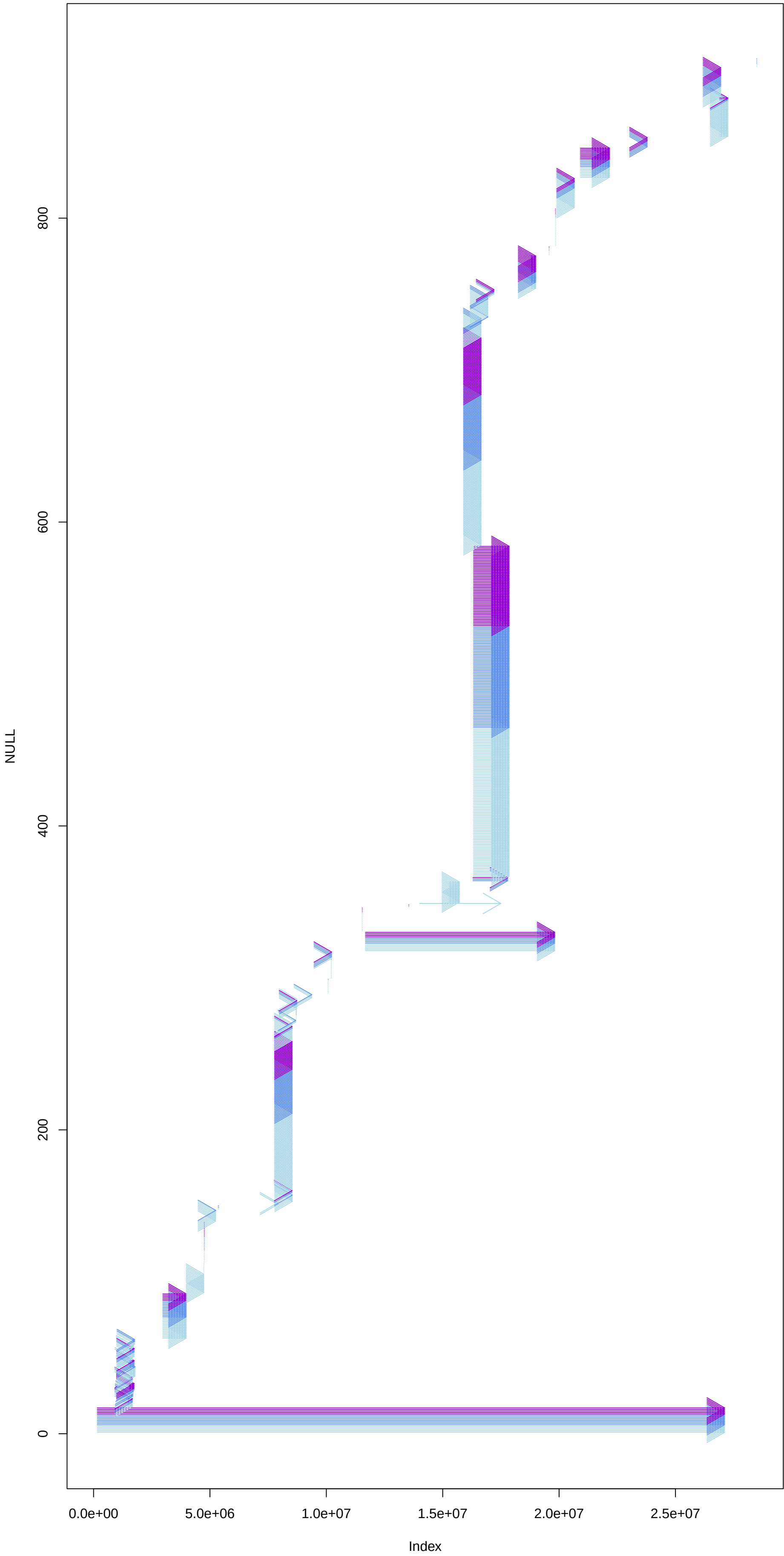
NC_044061.1 filtered 2 programs; 1 pass
