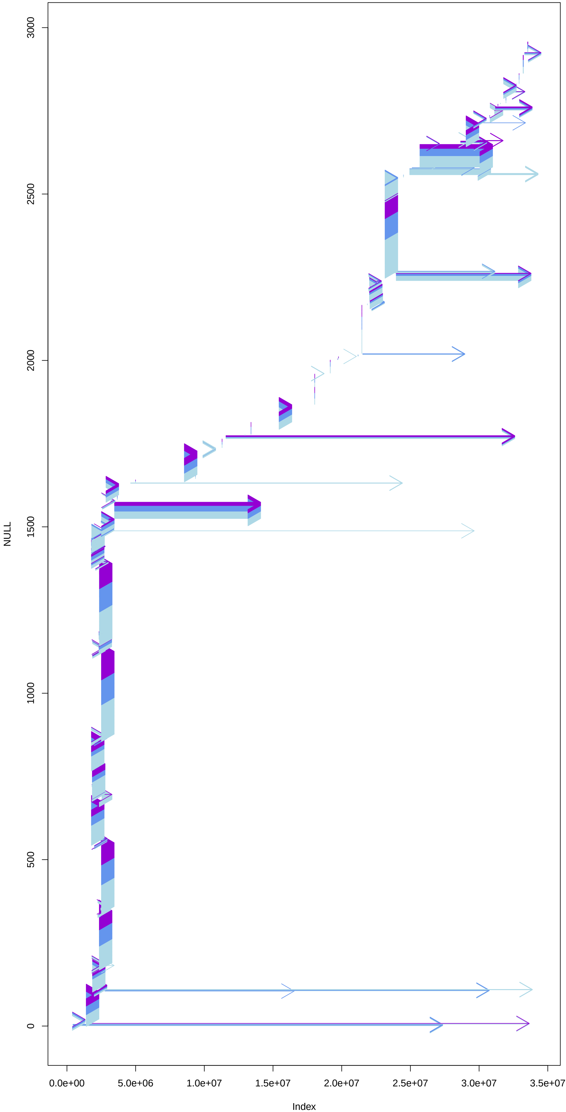
NC_044063.1 filtered 2 programs; 1 pass
