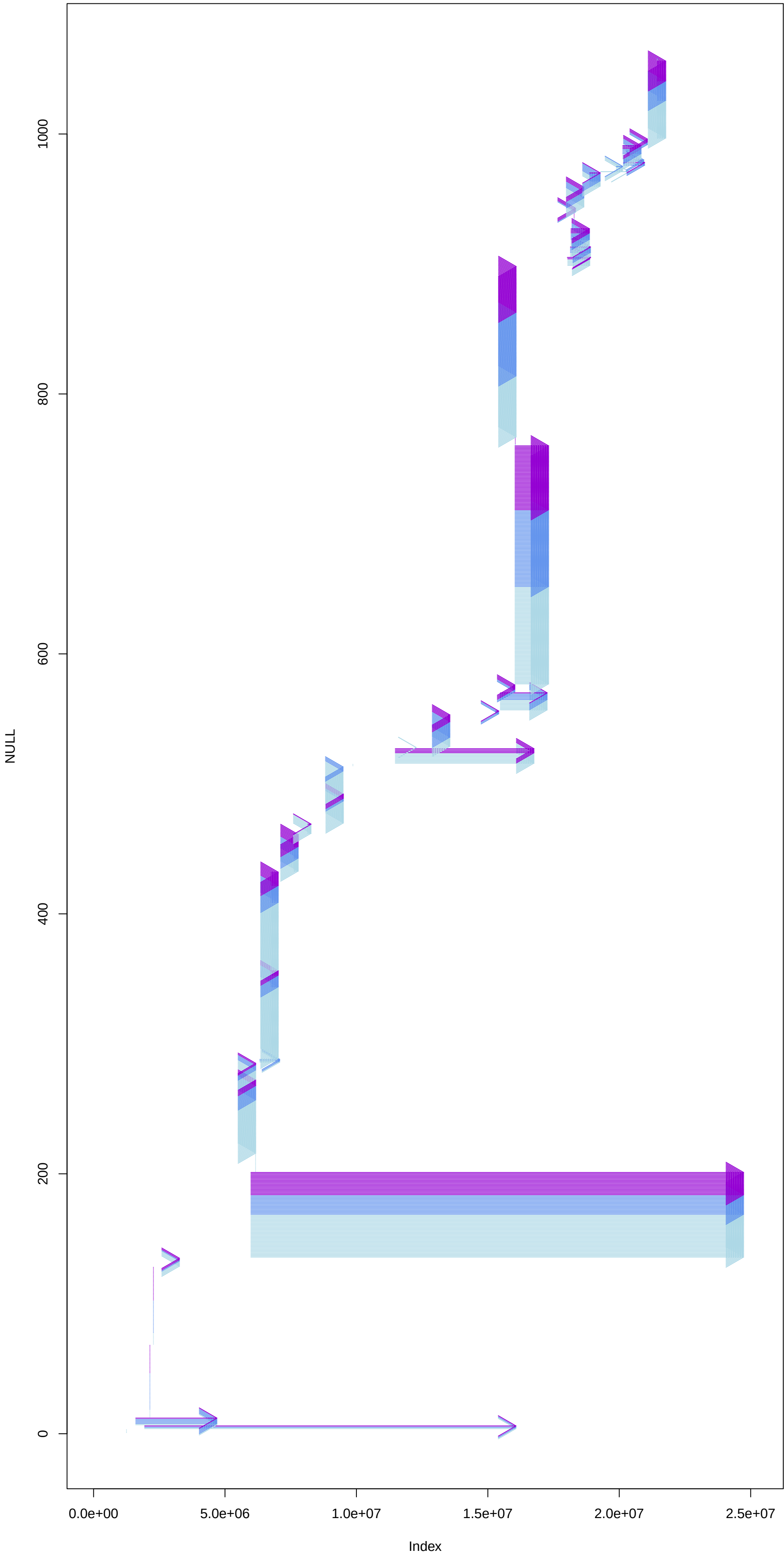
NC_044070.1 filtered 2 programs; 1 pass
