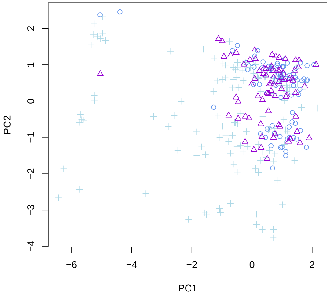
WindowID: 3; NC_044048.1 (LG 1); 99 SNPs
