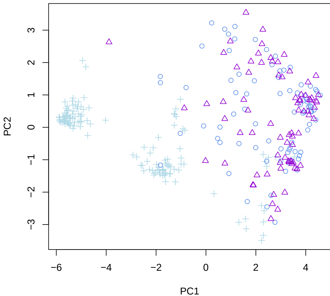
WindowID: 92; NC_044051.1 (LG 4); 99 SNPs
