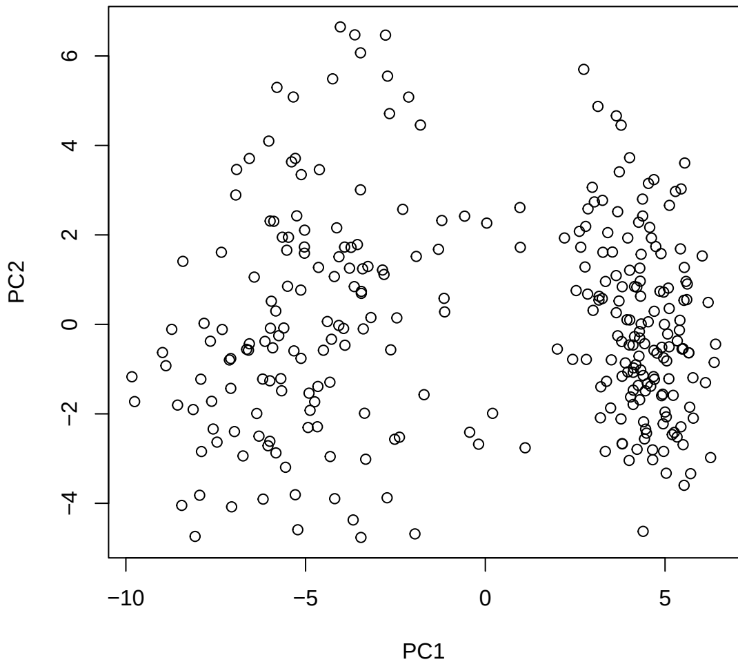
Window ID 14 NC_044049.1 (2)
