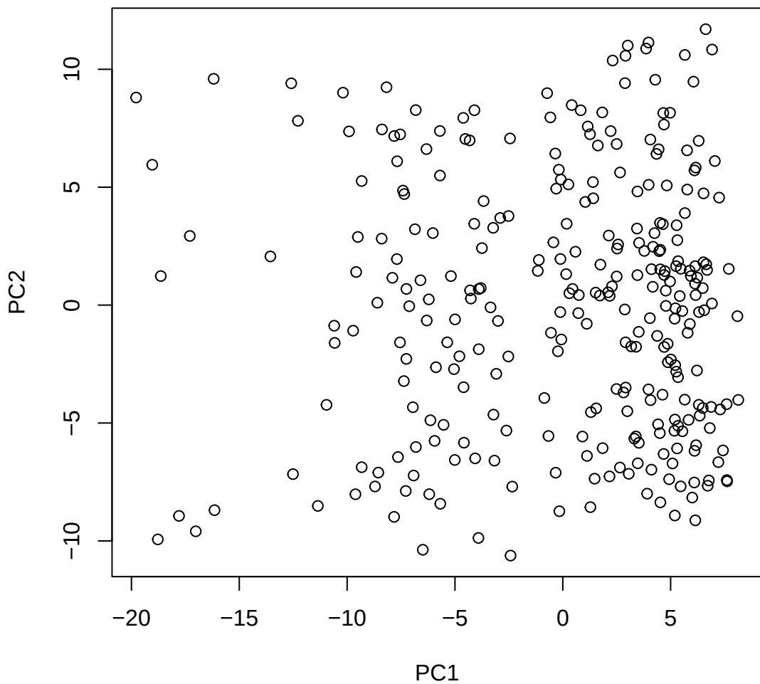
Window ID 21 NC_044050.1 (3)
