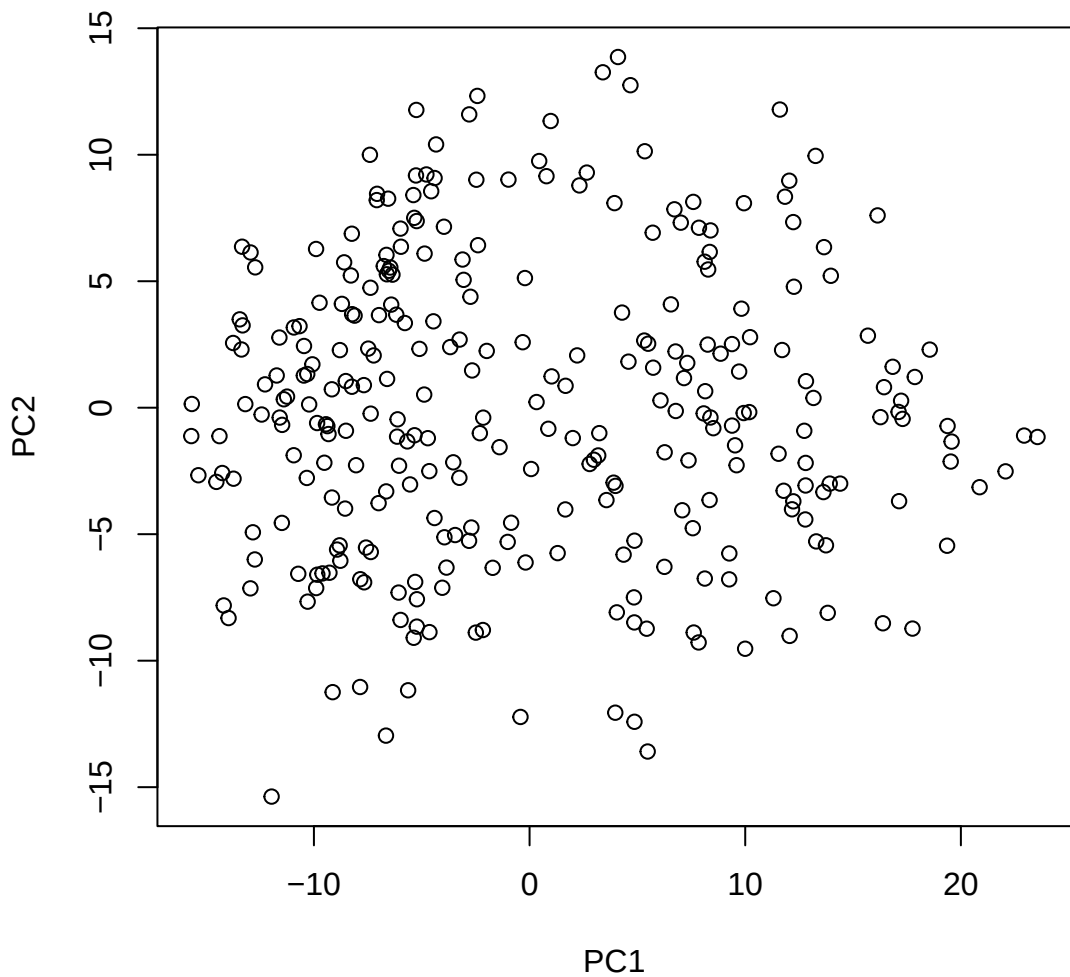
Window ID 78 NC_044055.1 (8)
