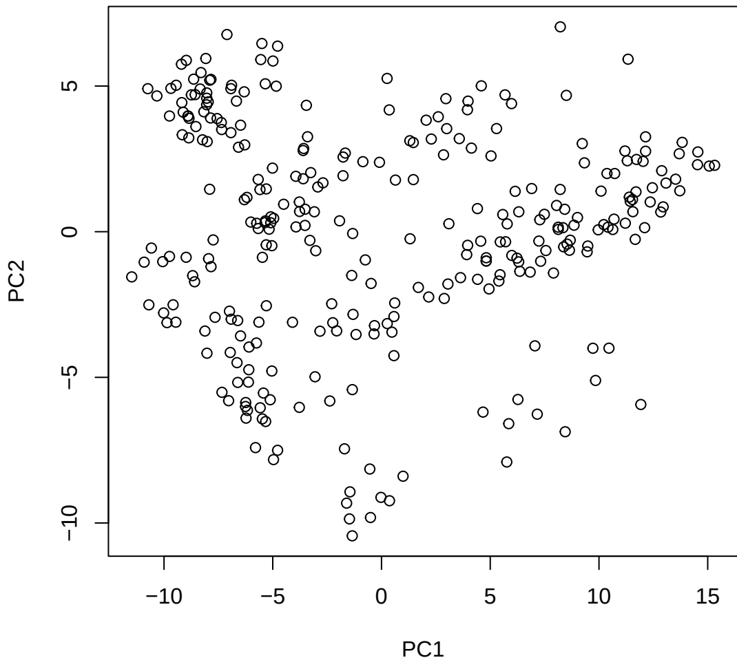
Window ID 137 NC_044062.1 (15)
