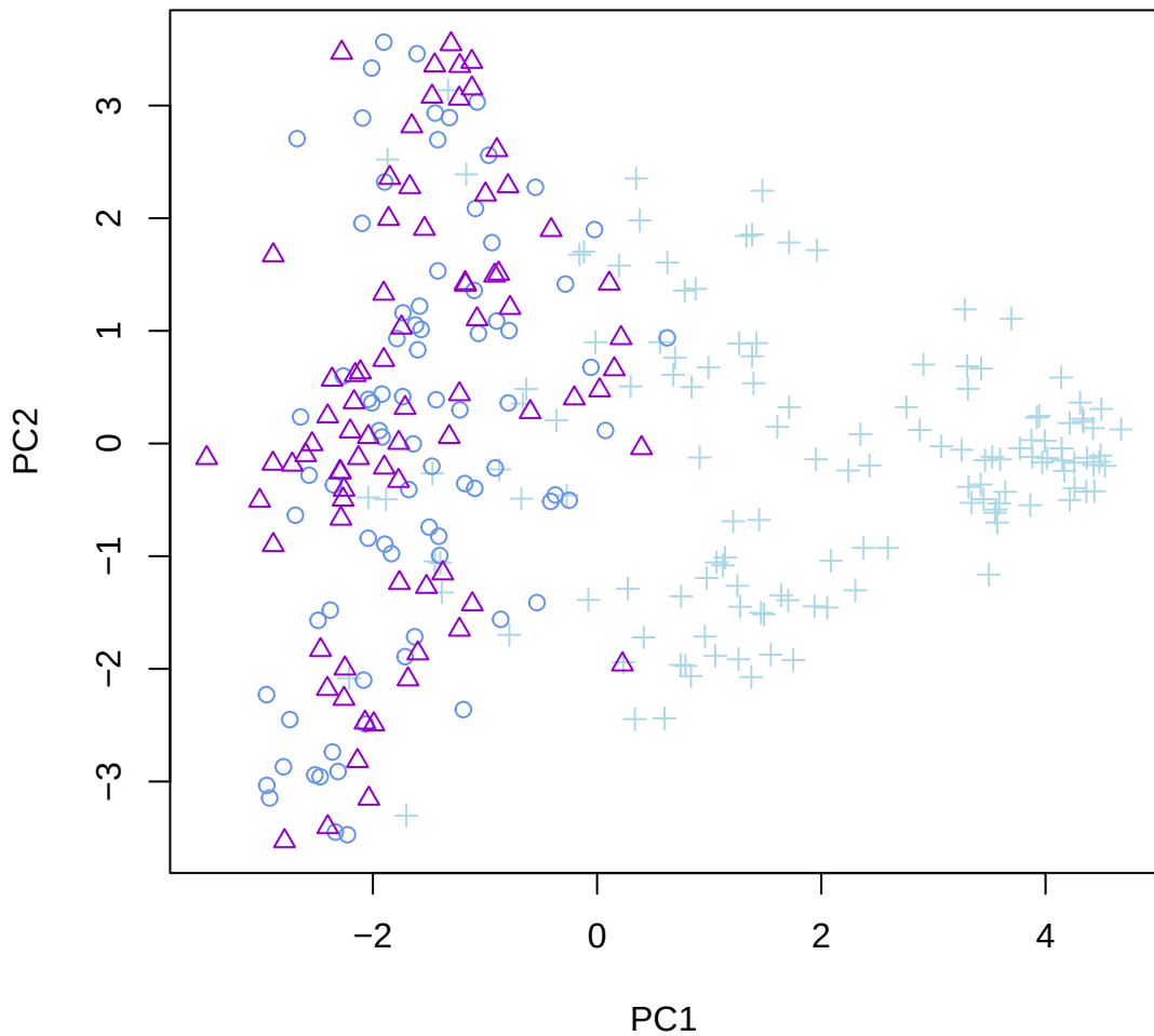
WindowID: 16; NC_044048.1 (LG 1); 99 SNPs
