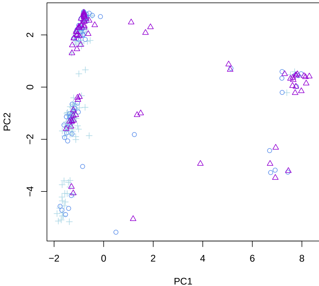
WindowID: 45; NC_044049.1 (LG 2); 99 SNPs
