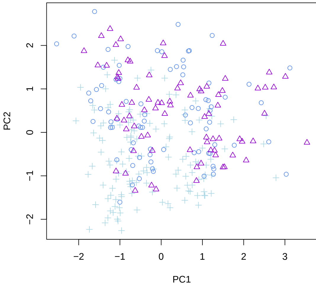
WindowID: 98; NC_044051.1 (LG 4); 99 SNPs
