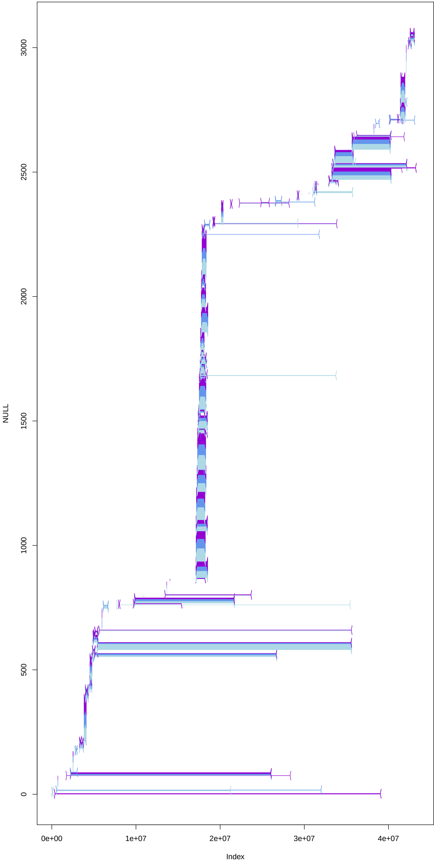
NC_044051.1 filtered 3 programs; 1 pass
