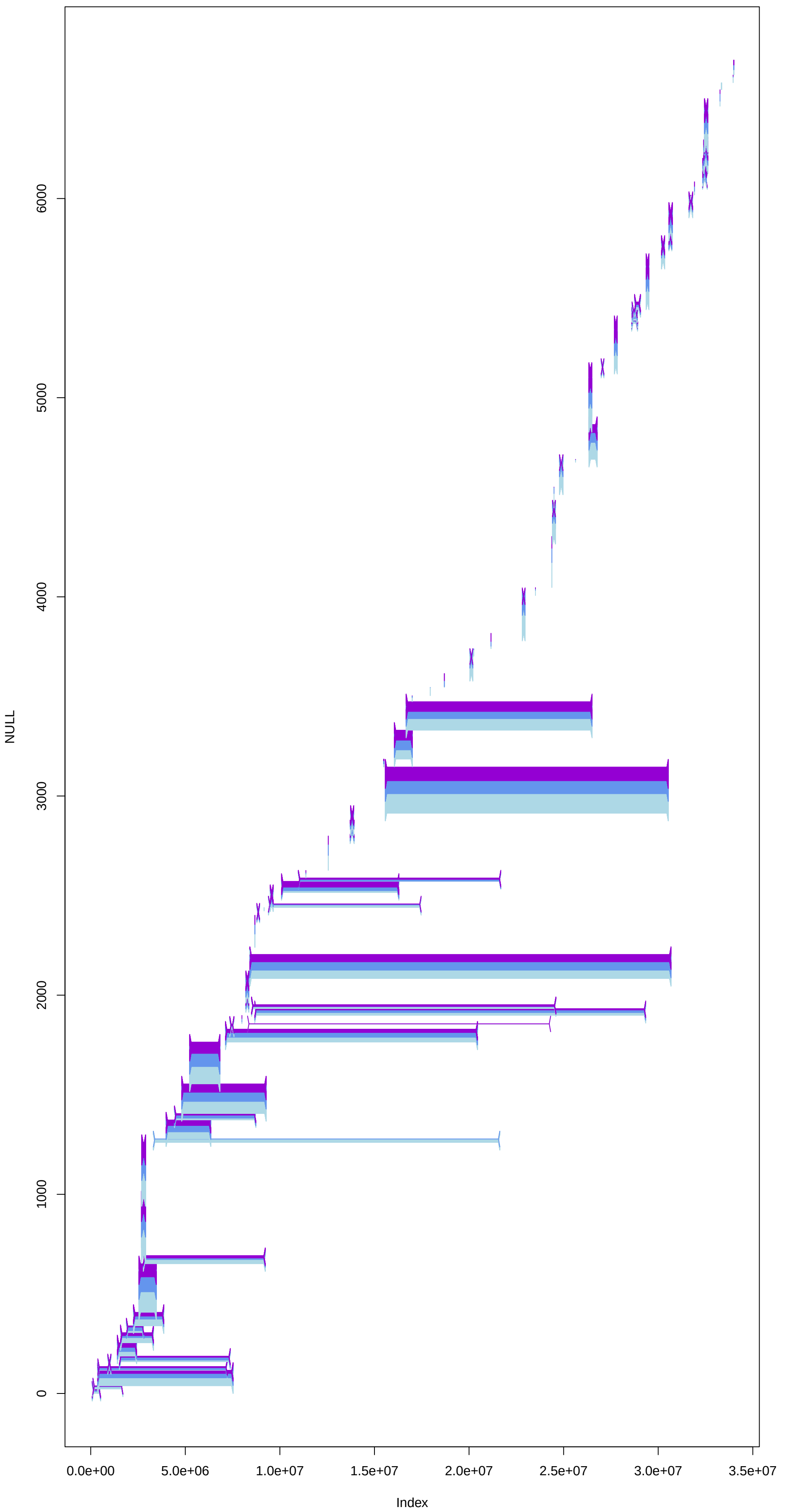
NC_044054.1
