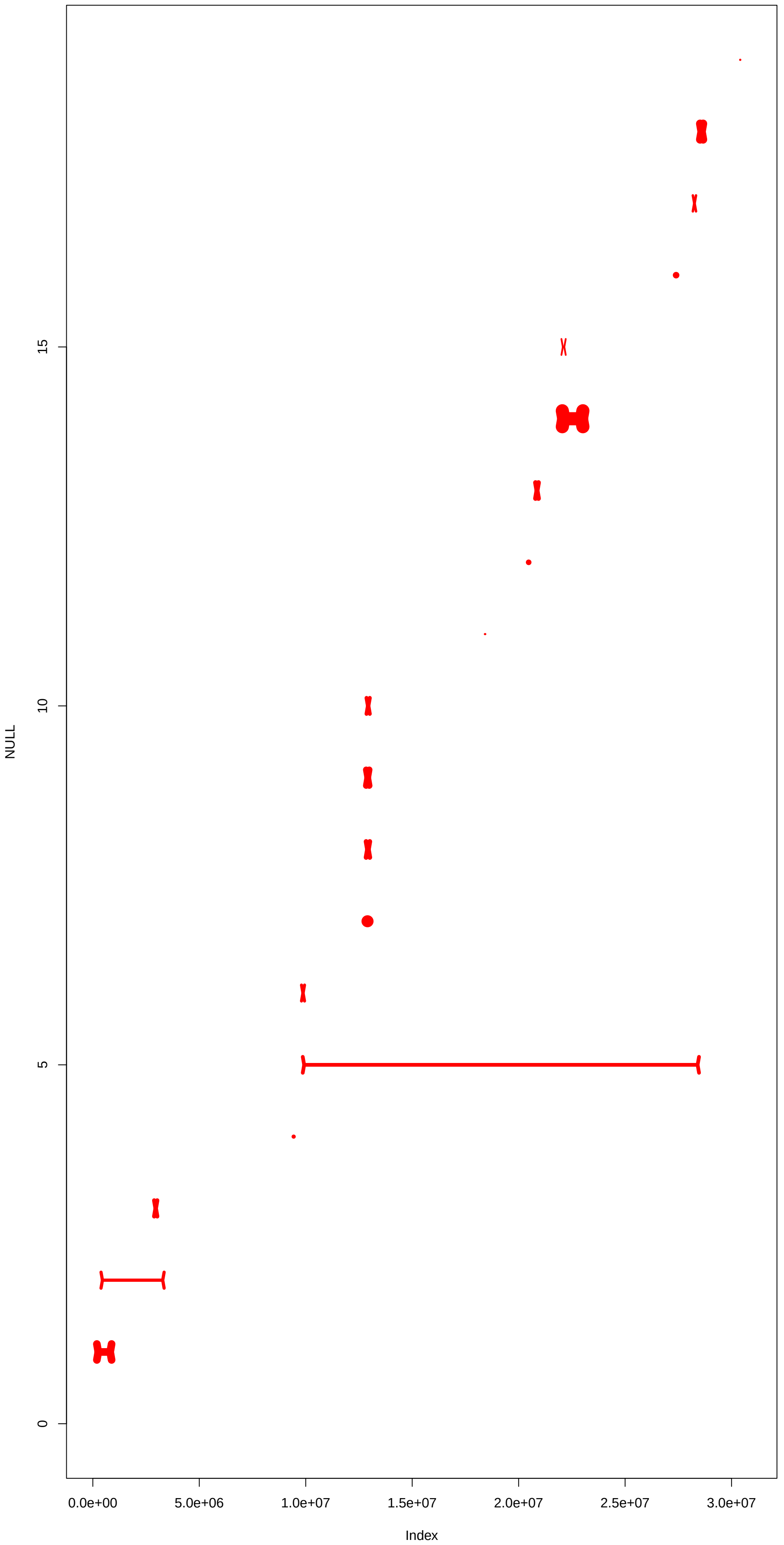
NC_044058.1 pass2
