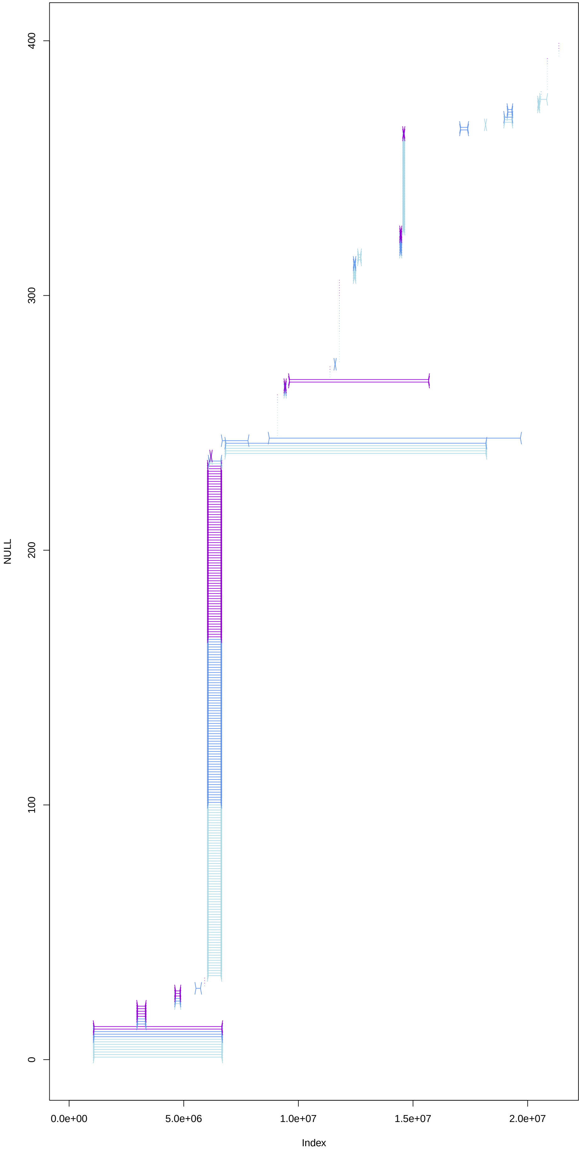
NC_044065.1 filtered 3 programs; 1 pass
