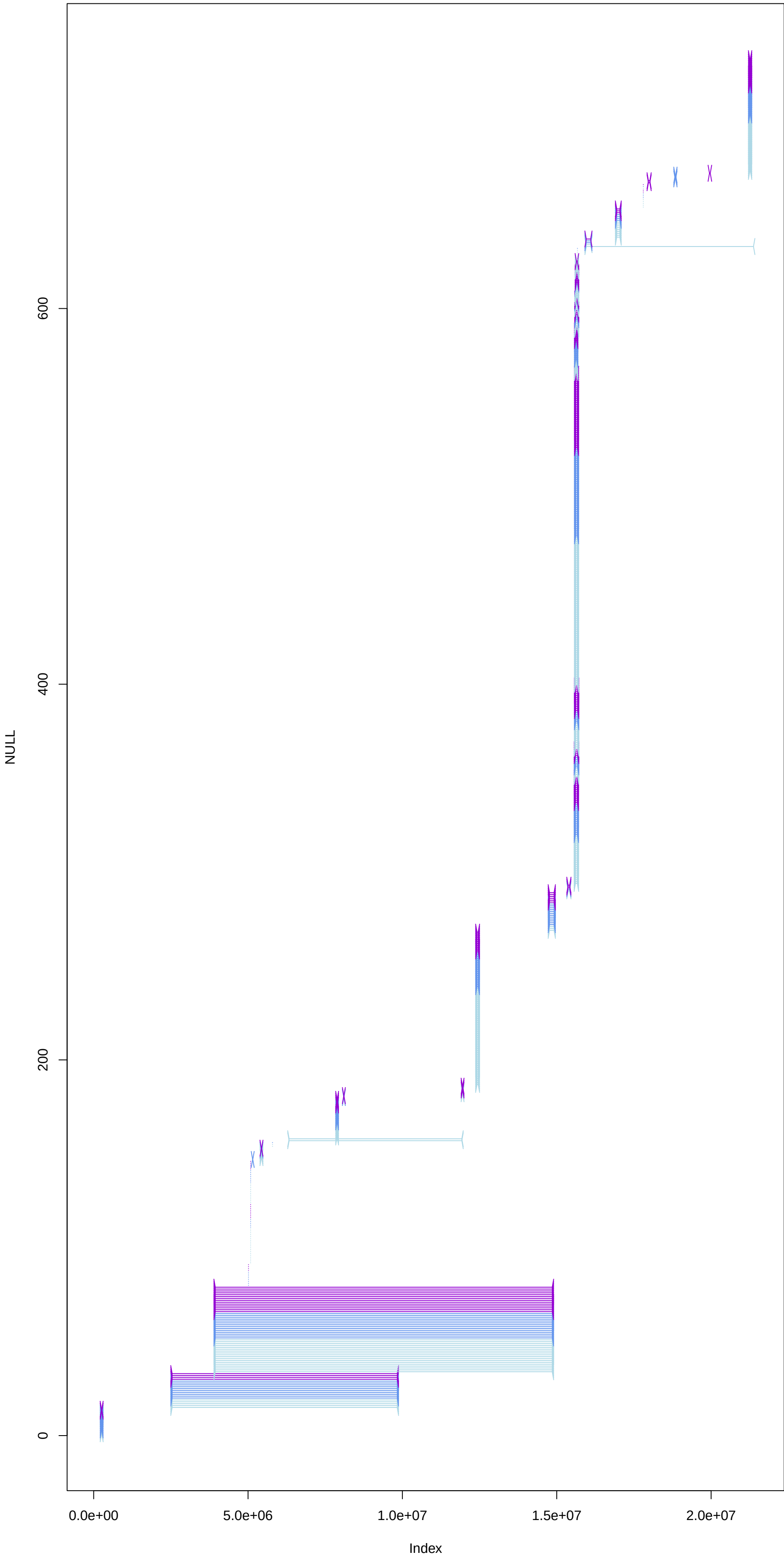
NC_044066.1 filtered 3 programs; 1 pass
