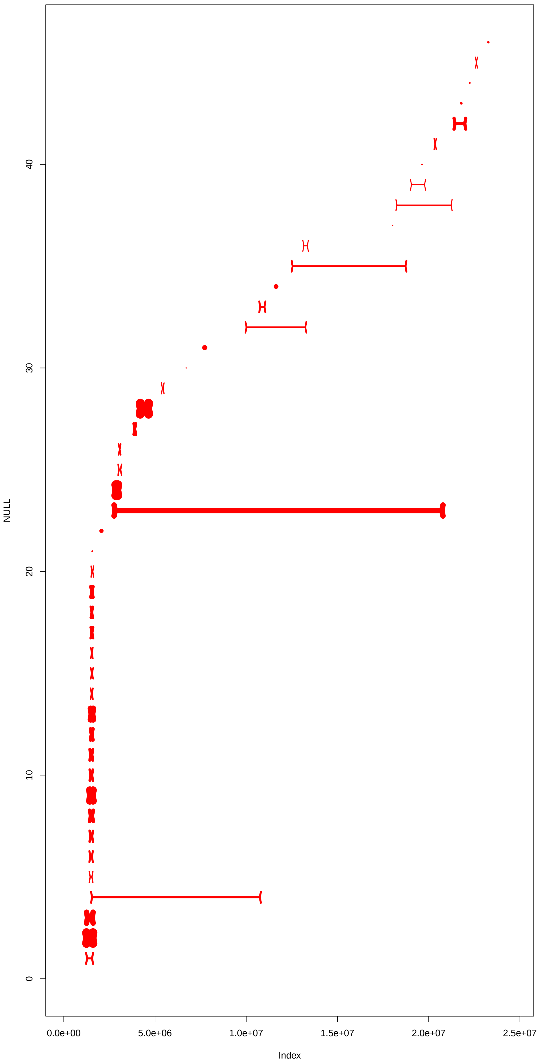
NC_044067.1 pass1
