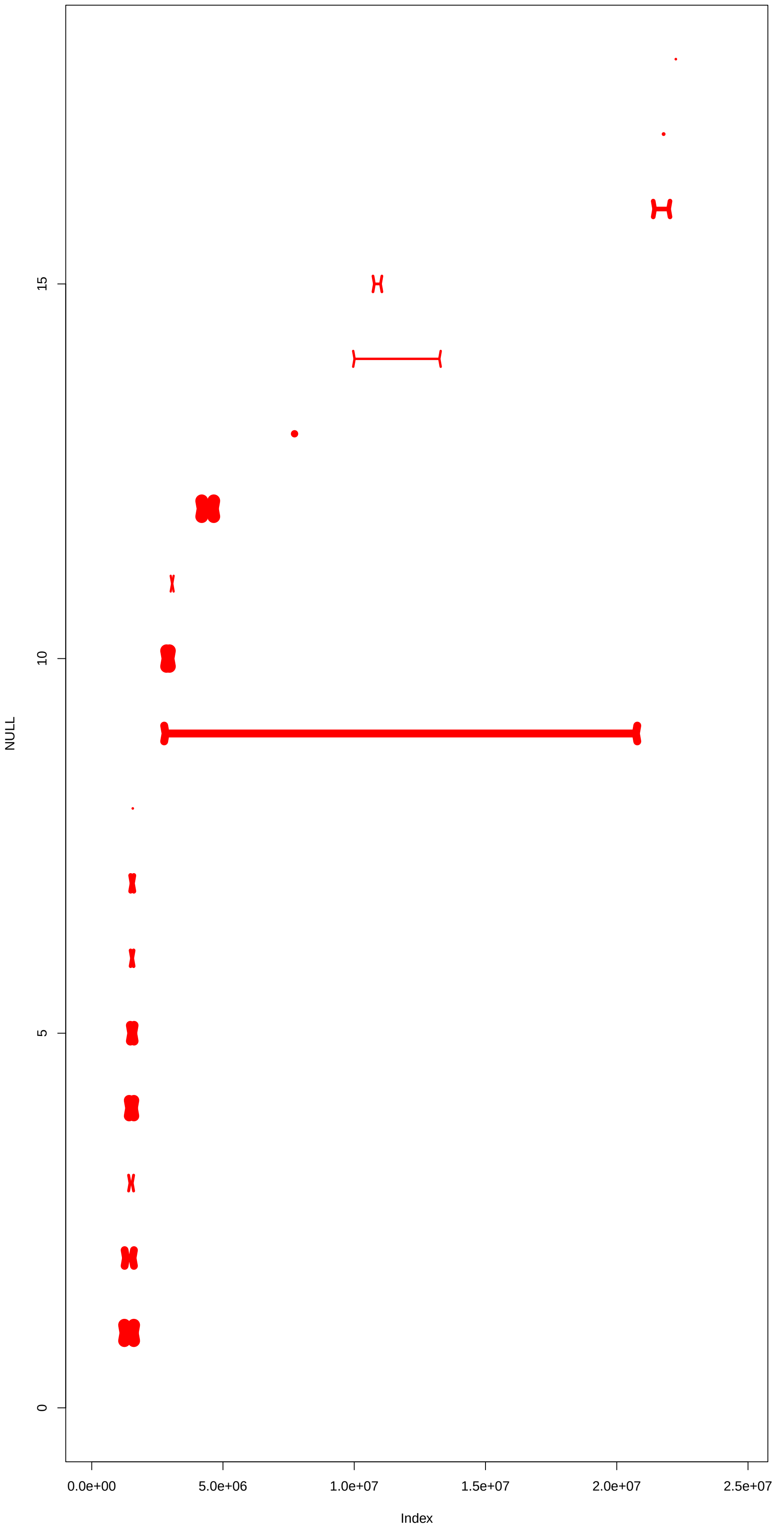
NC_044067.1 pass2
