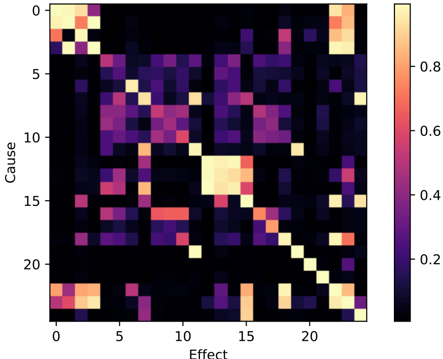
Causal matrix
