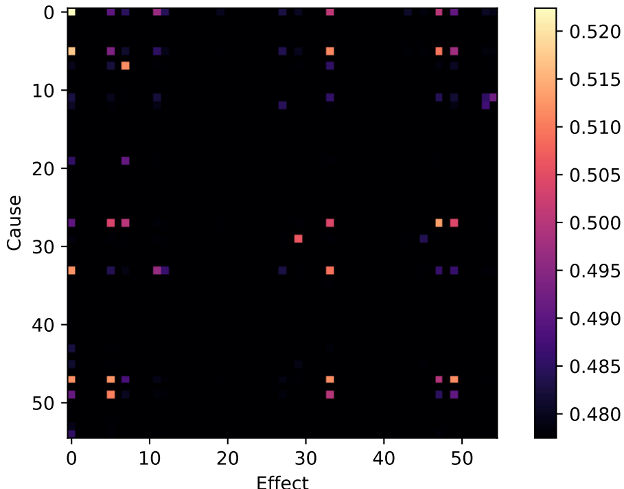
Causal matrix
