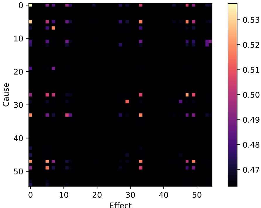
Causal matrix
