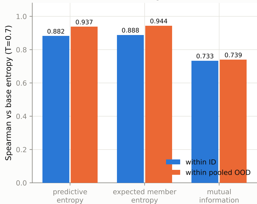
b How much of P&C's ranking is the base model's?
