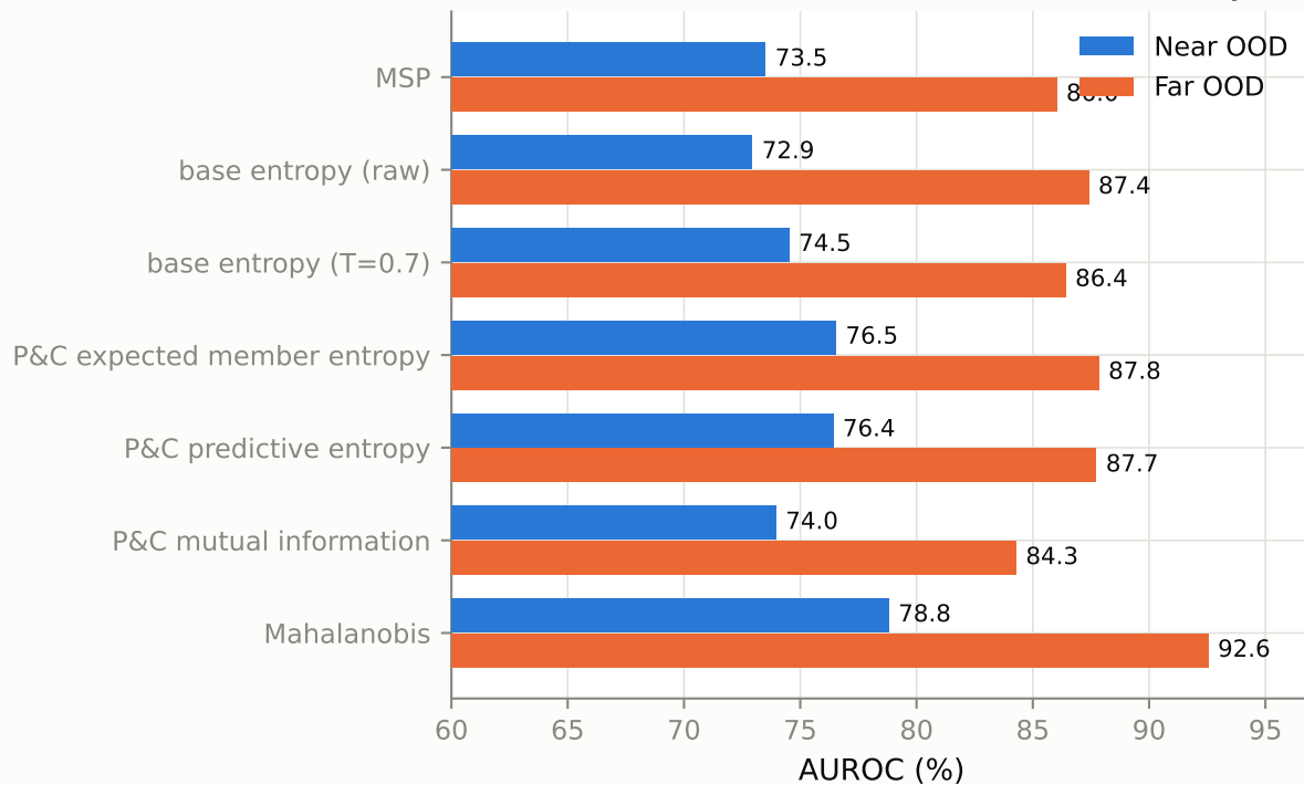
a Base confidence vs P&C ensemble uncertainty
