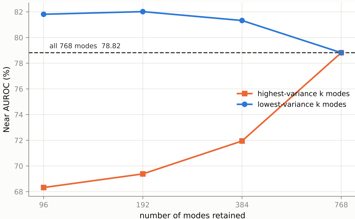
The lowest-variance 96 modes alone beat the full detector
