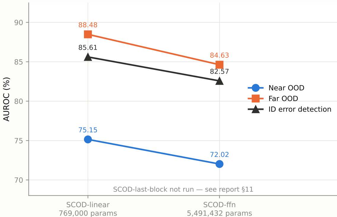
Enlarging the SCOD parameter scope makes it worse (k=30, exact Fisher)
