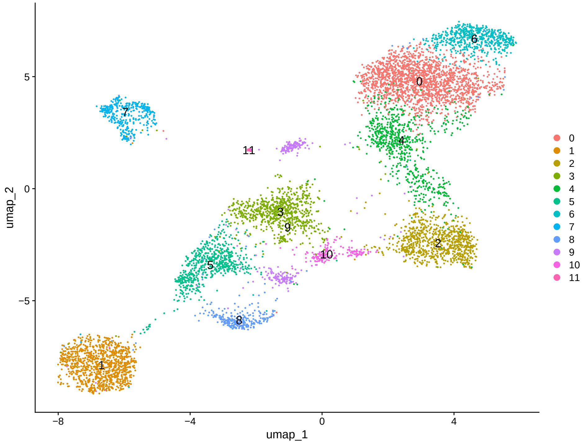
UMAP – All Cells Colored by Cluster
