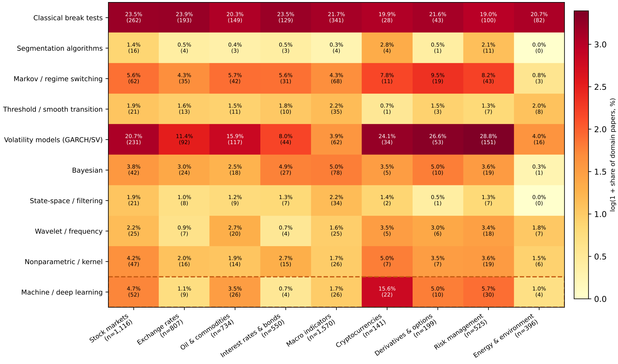
Detection papers mentioning each method family, by application domain (share of domain papers, count)
