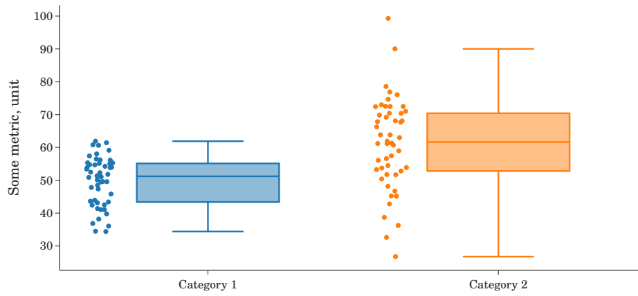
A plot of two random samples
