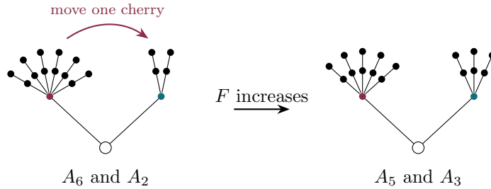
Figure 11: The balance move of Lemma 7, shown with k = 2, t = 2 (the centre's other children are not drawn). Whenever the centre has at least three children, evening out two arms whose sizes differ by two or more strictly increases the ratio. So a best spider has all its arms of two consecutive sizes.
