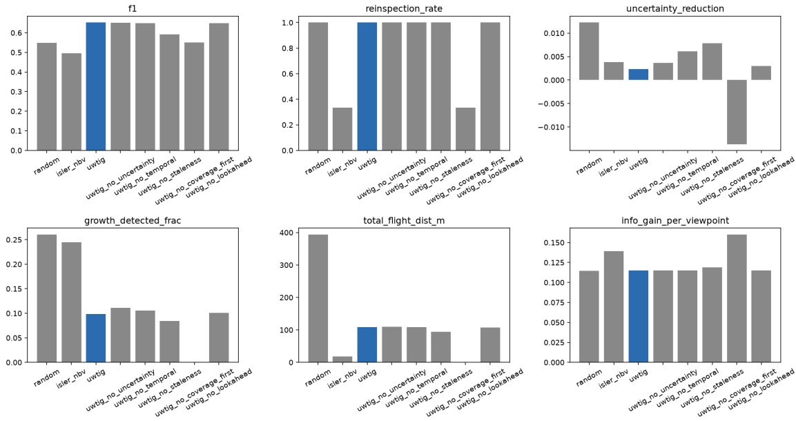
Figure 3. Comparison chart across all eight planners (blue = UW-TIG) for six of the logged metrics, generated directly by experiments/evaluate.py .
