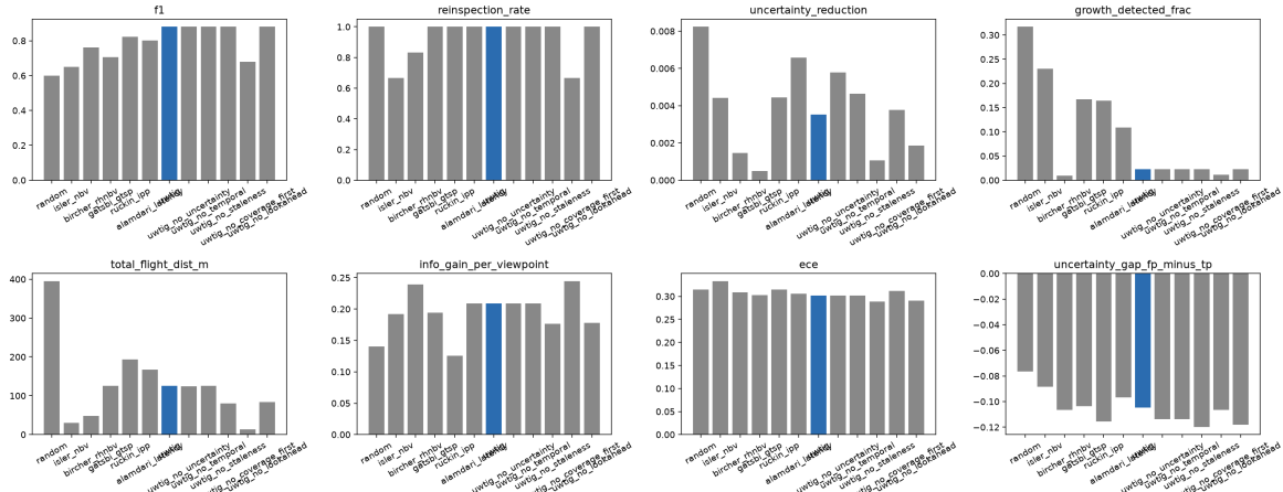
Figure 3. Comparison chart across all twelve planners (blue = UW-TIG) for the logged metrics, generated directly by experiments/evaluate.py .
