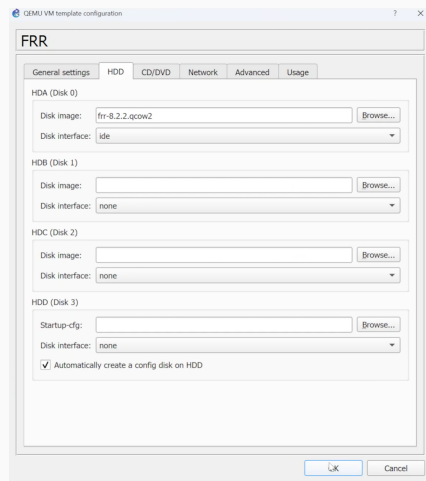
Рис. 27: Automatically create a config disk on hdd
