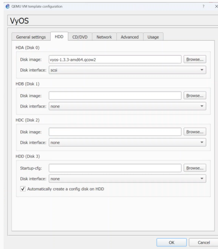
Рис. 35: Automatically create a config disk on hdd
