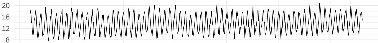
Seasonal
