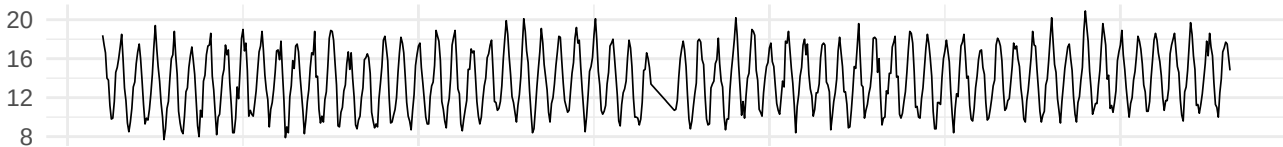
Spline
