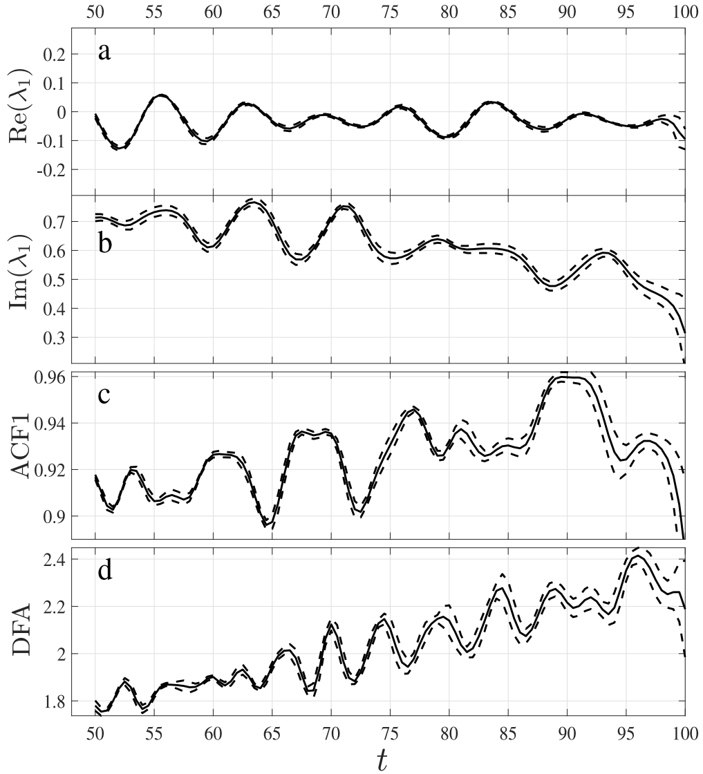
Fig. 3.2 Tipping point indicators applied to System A (equation 3.27) which experiences a homoclinic bifurcation at t = 100 . Panels a and b show the real and imaginary parts of the first reconstructed eigenvalue of the Jacobian matrix, as in equation 3.8. Panels c and d show the ACF1 and DFA indicators calculated with a window size of 100 points, applied to the one-dimensional time series obtained by applying EOF dimension reduction to the data. The system was integrated ten times and the mean over ten data sets is plotted, along with error of one standard deviation (dashed lines).
