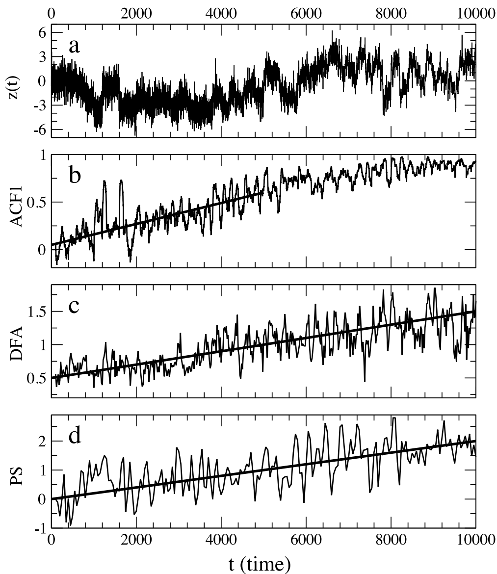
Fig. 2.11 Artificial data with ACF1, DFA and PS indicators. (a) A time series is constructed by concatenating 50 sub-series of length 200 where the scaling exponent \beta within each sub-series is constant and increases over the whole series from 0 (white noise) to 2. (b,c,d) The ACF1, DFA and PS indicator methods are applied with window size 100. As the PS-indicator increases from 0 to 2, the ACF indicator increases from 0 to 1, and the DFA indicator \alpha increases from 0.5 to 1.5. Lines are added to show the linear trends; note that the ACF indicator does not increase linearly as it approaches 1.
