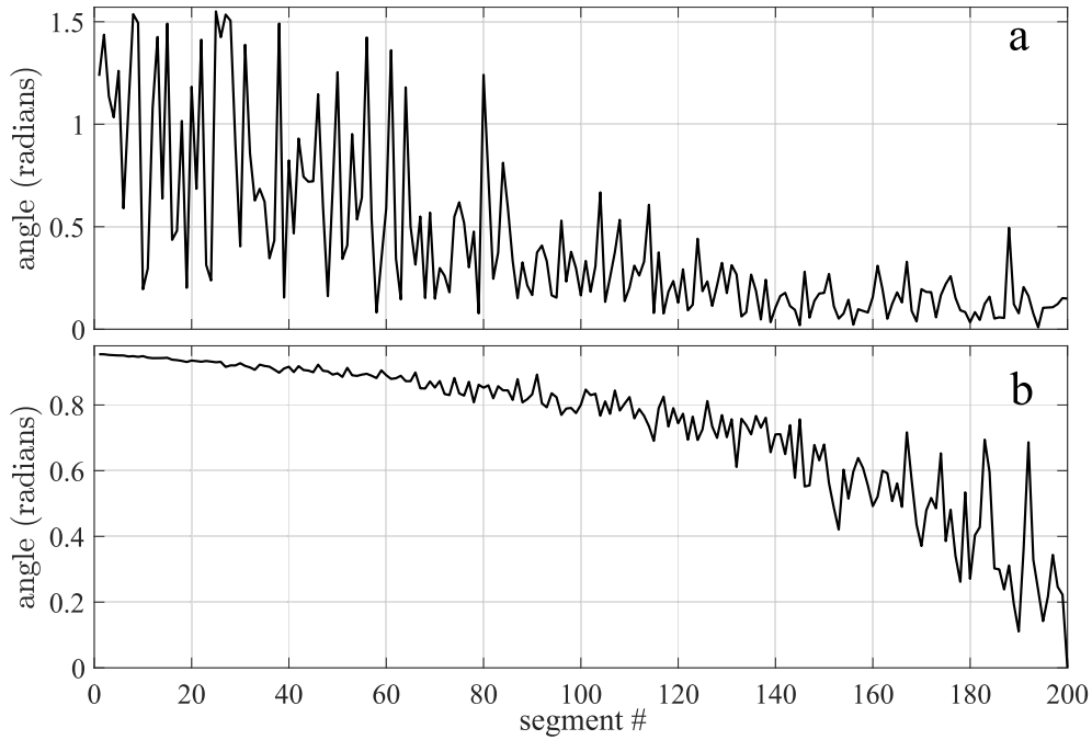
Fig. 3.11 The angle variable of the EOF eigenvector calculated in 200 overlapping segments of length 10^3 . Two cases of the three-dimensional system in equation 3.91 are considered: using S_1 (panel a ) and using S_2 (panel b ).
