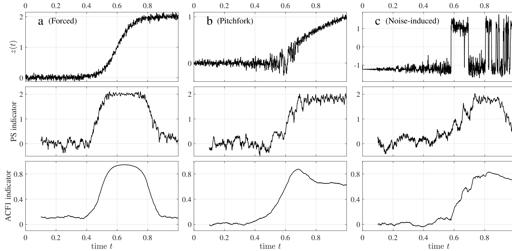
Fig. 2.12 Three systems given by equations 2.99 (forced transition), 2.100 (pitchfork bifurcation), and 2.101 (noise-induced tipping point) are integrated between t = 0 and t = 1 . Each exhibits a tipping point at around t = 0.6 : a forced transition, a pitchfork bifurcation, and a noise-induced transition (panels a, b, c resp.). The PS and ACF1 indicators are calculated using a sliding window of 100 points and plotted beneath the time series for each system. We note the similarity in shape between the two indicator signals, although the PS indicator is more noisy.
