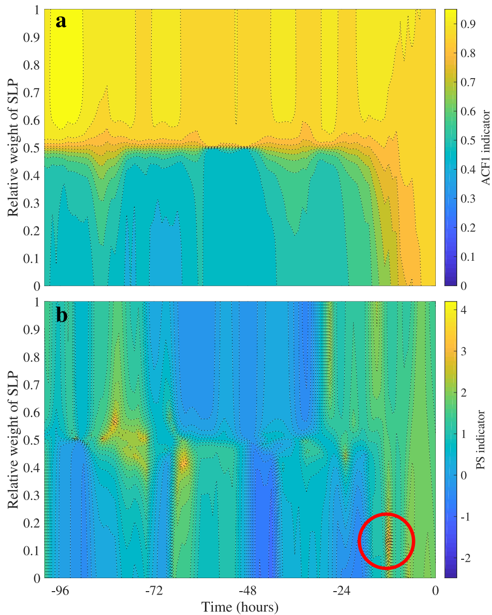
Fig. 4.12 Sensitivity of the ACF1 and PS indicators to different EOF weighting schemes. The widowed EOF projection is found for a range of SLP weighting values from p = 0 (only wind speed considered) to p = 1 (only SLP considered) and the ACF1 and PS indicators are calculated (panels a and b respectively). A non-periodic spike in the PS indicator is circled in red.
