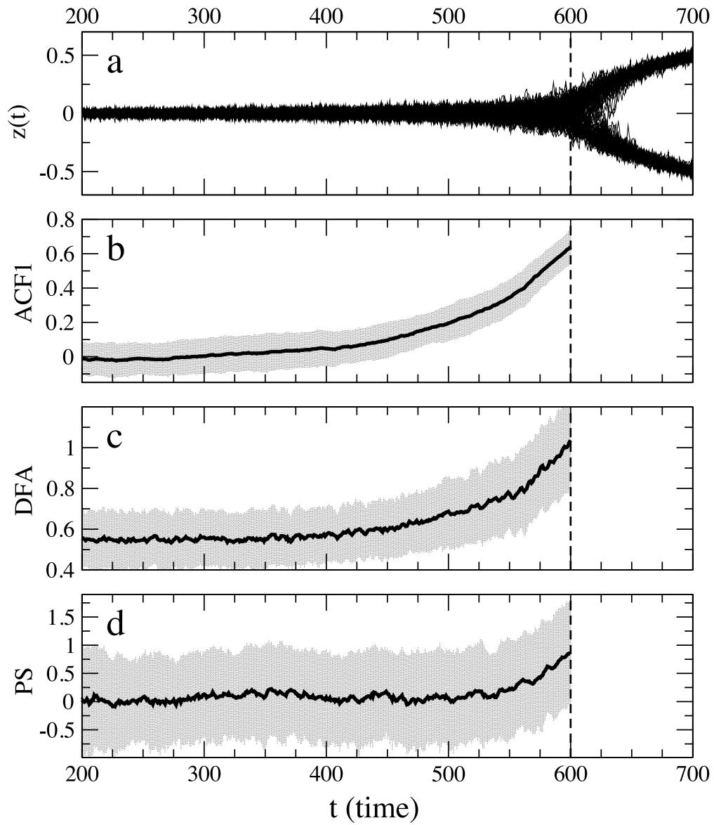
Fig. 2.14 ACF1, DFA and PS indicators applied to model data. (a) Data from 100 runs of the model (see eq. 2.105); (b,c,d) The mean ACF1, DFA and PS indicators (window size 100) shown with error bars of one standard deviation. The values of all the indicators begin to rise before the bifurcation, as expected, at around t = 500 , although it is most noticeable for the ACF1 indicator.
