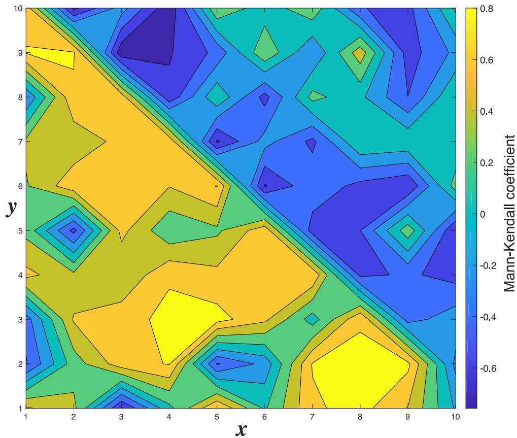
Fig. 3.17 A 2D bifurcation caused by an approaching front. At each point (x, y) a system is described by equation 3.119 where the value of \mu is decreasing. The figure shows the Mann-Kendall coefficient of the ACF1 indicator of the series when \mu = 10 , when the bifurcation is occurring at points on the line y + x = 10 . To the top-right of this line, the bifurcation has already occurred and the lag-1 ACF is decreasing (negative Mann-Kendall coefficient). To the bottom-left of this line, the systems have not yet bifurcated and the ACF1 indicator is increasing (positive Mann-Kendall coefficient) as an EWS of the tipping point.
