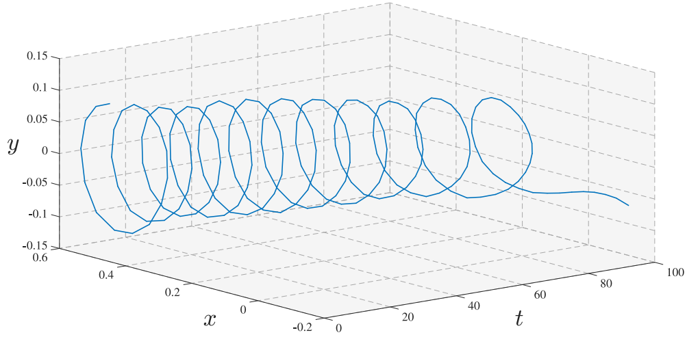
Fig. 3.1 A single realisation of the system in equation 3.27 with initial point (\sqrt{0.2}, 0.1) . The system spirals around the moving centre at (\sqrt{\alpha}, 0) , \alpha is given in equation 3.29, until t = 100 , \alpha = 0 , when the bifurcation occurs and the system tends towards infinity in the negative x and negative y directions.
