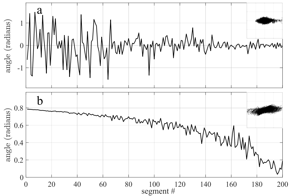
Fig. 3.9 The angle variable of the EOF eigenvector calculated in 200 overlapping segments of length 10^3 . Two cases of the system in equation 3.91 are considered: using S_1 (panel a ) and using S_2 (panel b ), see equations 3.93 and 3.94. The series itself is plotted, in each case, in the insert at the top-right of the panel, both x and y axes range from -2 to 2 .
