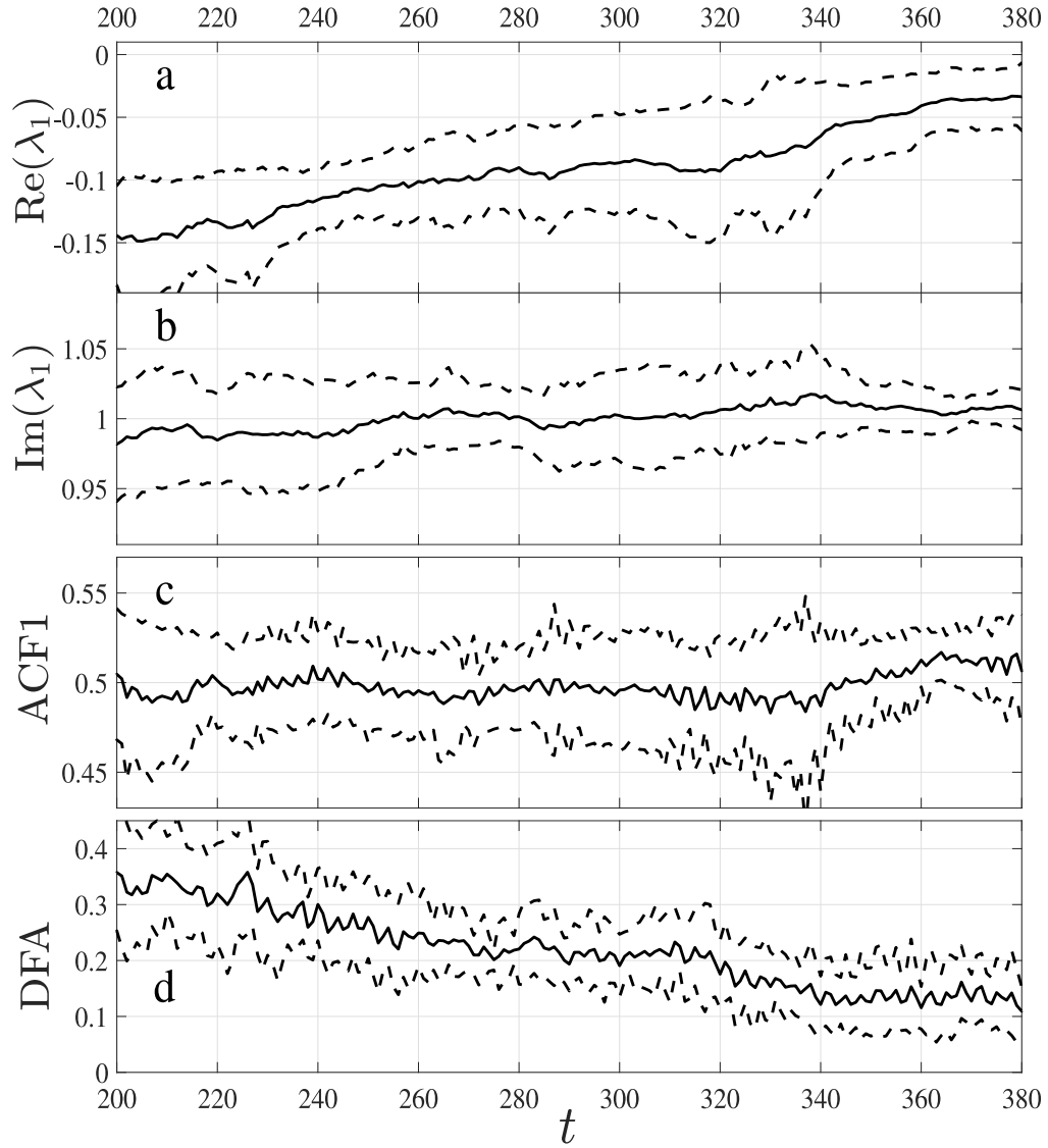
Fig. 3.6 Tipping point indicators applied to System C, the Van de Pol oscillator (equation 3.37), which experiences a Hopf bifurcation at t = 380 . Panels a and b show the real and imaginary parts of the first reconstructed eigenvalue of the Jacobian matrix, as in equation 3.8. Panels c and d show the ACF1 and DFA indicators calculated with a window size of 100 points, applied to the one-dimensional time series obtained by applying EOF dimension reduction to the data. The system was integrated ten times and the mean over ten data sets is plotted, along with error of one standard deviation (dashed lines).
