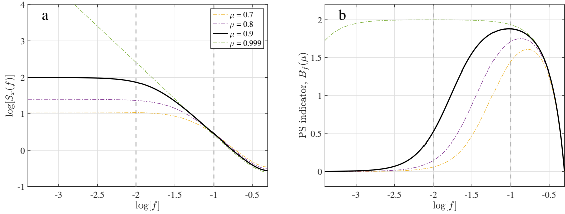
Fig. 2.9 (a) The power spectrum of the AR(1) process (see eqn. 2.81) is plotted on a log-log scale for various values of the parameter \mu . Note the ‘white-noise’ (flat) part of the power spectrum for small f and the ‘red-noise’ (negative gradient) part for large f . (b) The PS indicator (see eqn. 2.84) is plotted as a function of f for the same \mu values.
