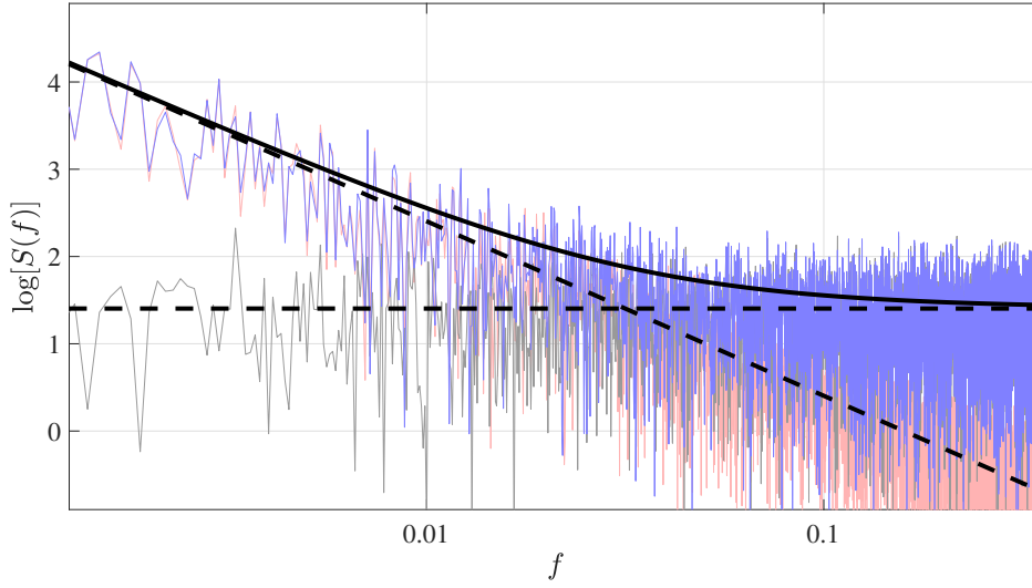
Fig. 2.7 Scaling crossover in the power spectrum of the sum of red and white noise series. Showing the power spectrum of the series z(t) (solid black line, see eqn. 2.68) imposed over the periodogram (blue). Also showing the power spectrum of white and red noise (dashed black lines) and their periodograms (grey and red resp.). The crossover occurs at f = 10^{-3/2} (see eqn. 2.76).
