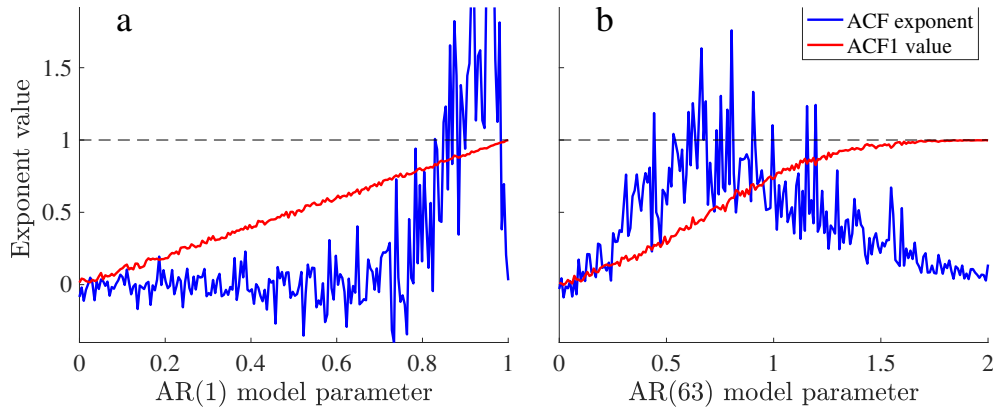
Fig. 2.5 ACF scaling exponent and the simple lag-1 ACF for 200 short-range correlated noise series (panel a), and 200 long-range correlated noise series (panel b), with varying correlation parameters.
