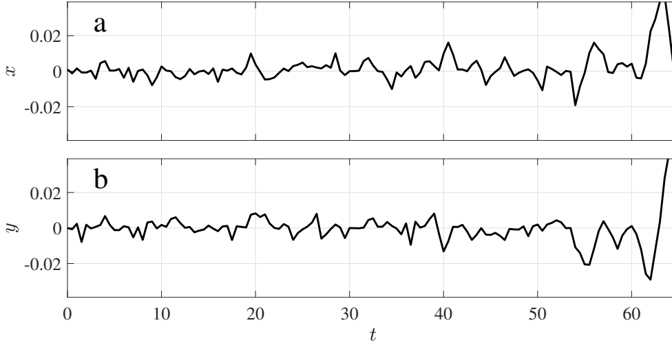
Fig. 3.3 A single realisation of the system in equation 3.35 with initial point (0,0) . The system oscillates about the stable point (0,0) until t = 58 when the bifurcation occurs and the stability is lost.
