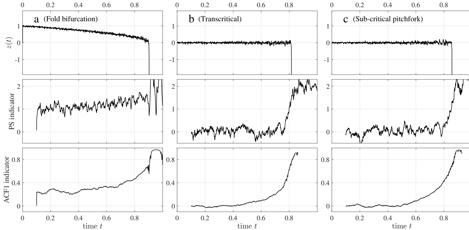
Fig. 2.13 Three systems given by equations 2.102 (fold bifurcation), 2.103 (transcritical bifurcation), and 2.104 (sub-critical pitchfork bifurcation) are integrated between t = 0 and t = 1 . Each exhibits a bifurcation at around t = 0.9 : a fold, transcritical, and sub-critical pitchfork bifurcation (panels a, b, c resp.). The PS and ACF1 indicators are calculated using a sliding window of 100 points and plotted beneath the time series for each system. We note the similarity in shape between the two indicator signals, although the PS indicator is more noisy.
