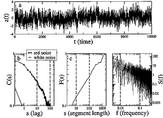
Fig. 1: Analysis of artificial red noise with scaling exponents measured using three different methods. (a) Red noise with a power spectrum scaling exponent of 0.85. (b) The ACF of the red noise data is calculated for different lags and the exponent (negative slope) measured in the range 10 \leq s \leq 100 (dashed lines). We note that the ACF(1)-indicator ( C(1) ) is 0.64. The ACF of a white noise series is also plotted for comparison, in this case C(s) = 0 for s \geq 1 and the exponent is also zero. (c) DFA calculated for the data and the exponent (slope) measured in the range 10 \leq s \leq 100 . (d) The power spectrum of the data, and the exponent (negative slope) measured in the frequency range 10^{-2} \leq f \leq 10^{-1} .
