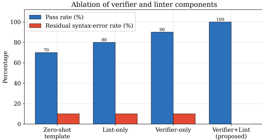
Figure 7. Ablation of the verifier and linter. The pass rate rises from 70% for open-loop generation to 100% when both guards and the repair loop are active, while the residual syntax-error rate falls to zero.
