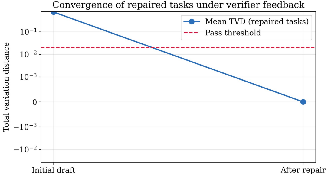
Mean total variation distance of the repaired tasks before and after the repair step (symmetric-log axis). Feedback-driven regeneration drives the distance from order 10^{-1} to machine epsilon in one iteration.
