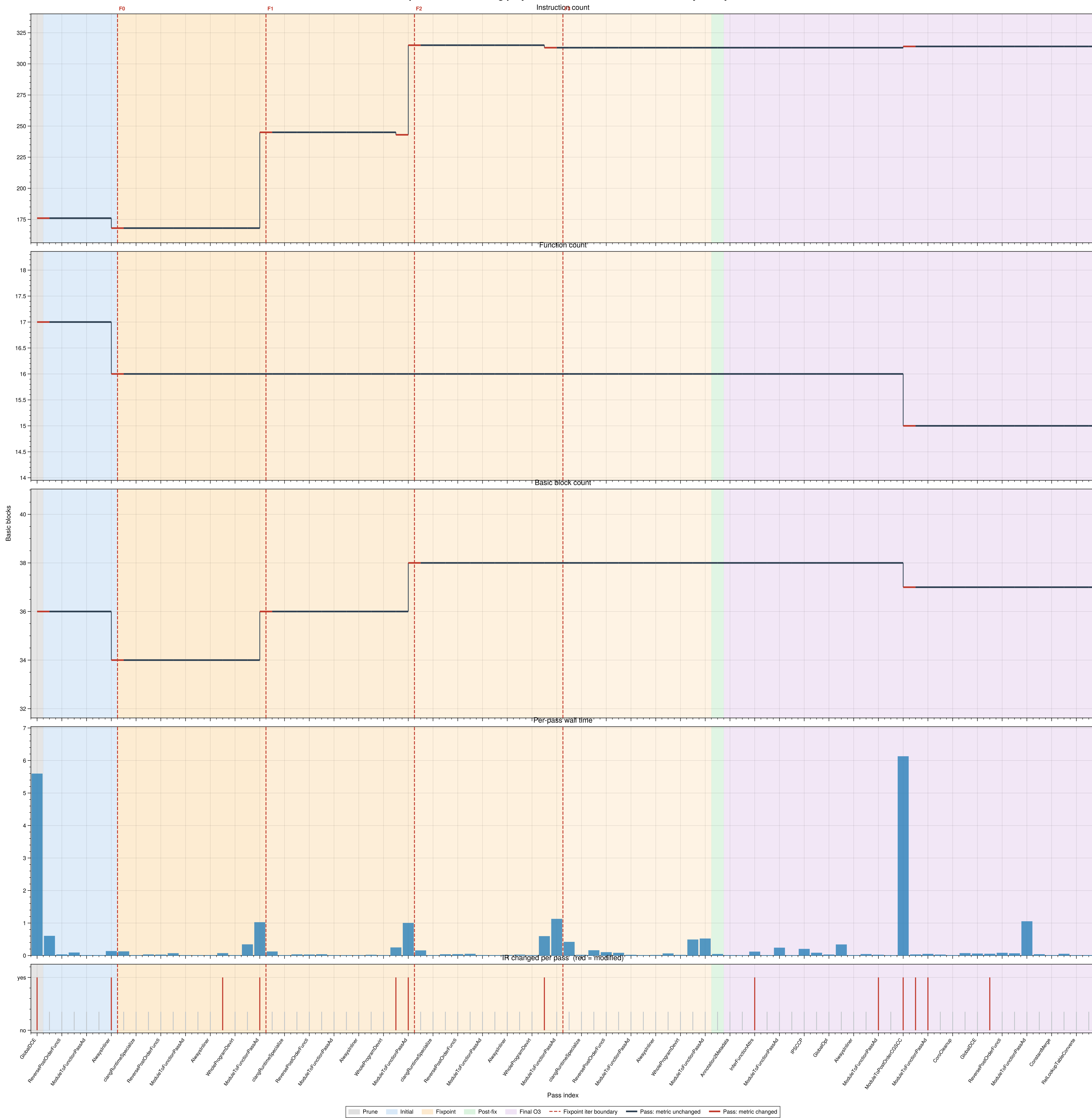
JIT Pipeline Trace — BM g polybench n seidel 2d s EXTRALARGE t jit analysis
