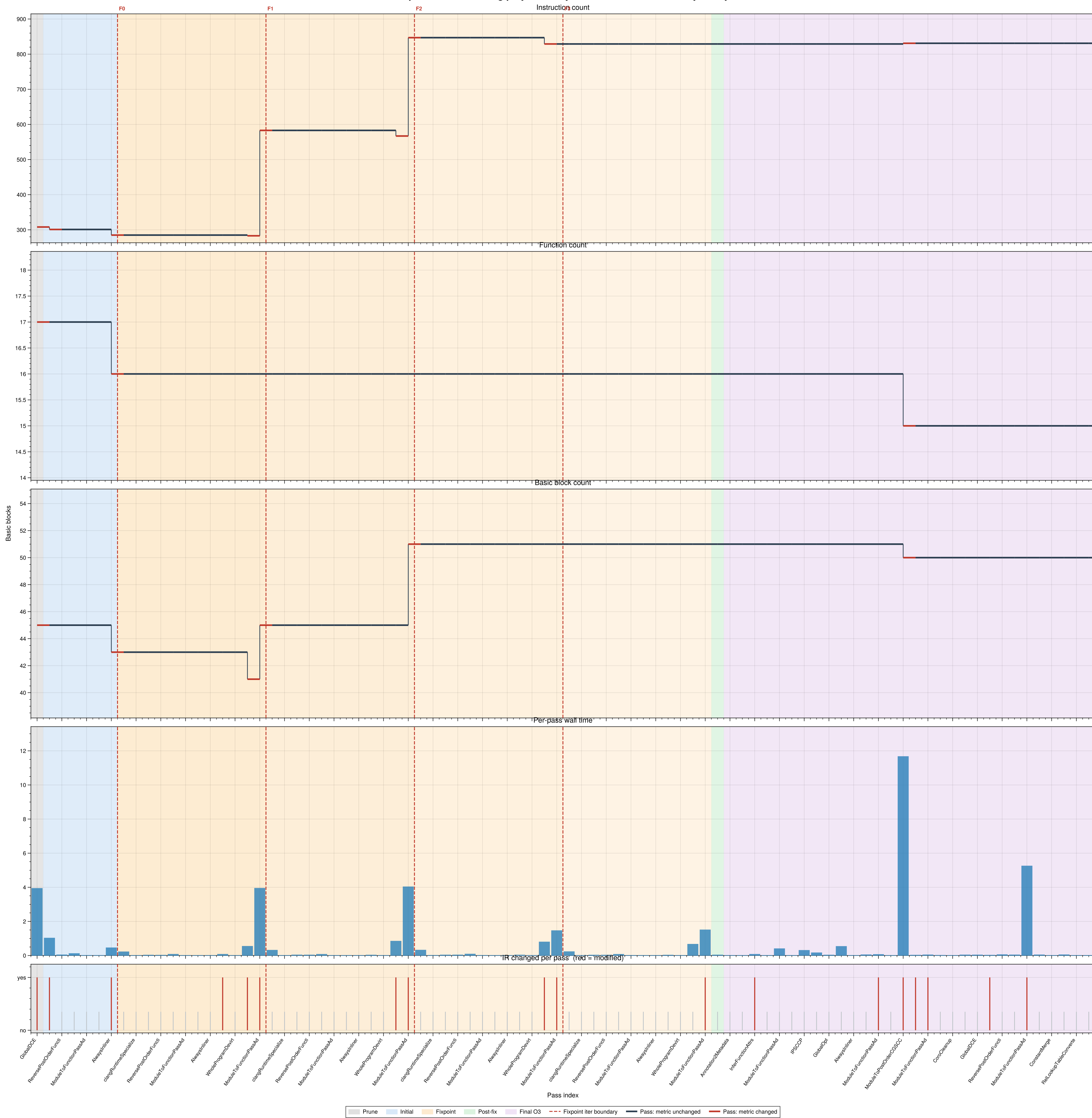
JIT Pipeline Trace — BM g polybench n jacobi 2d s EXTRALARGE t jit analysis
