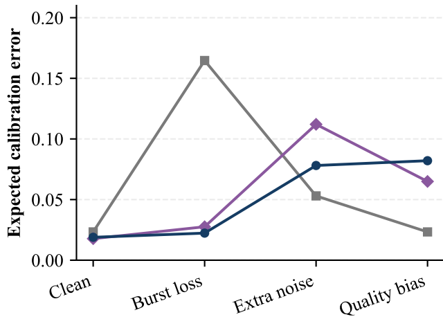
(b) Calibration error
