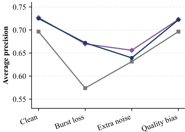
(a) Discrimination
