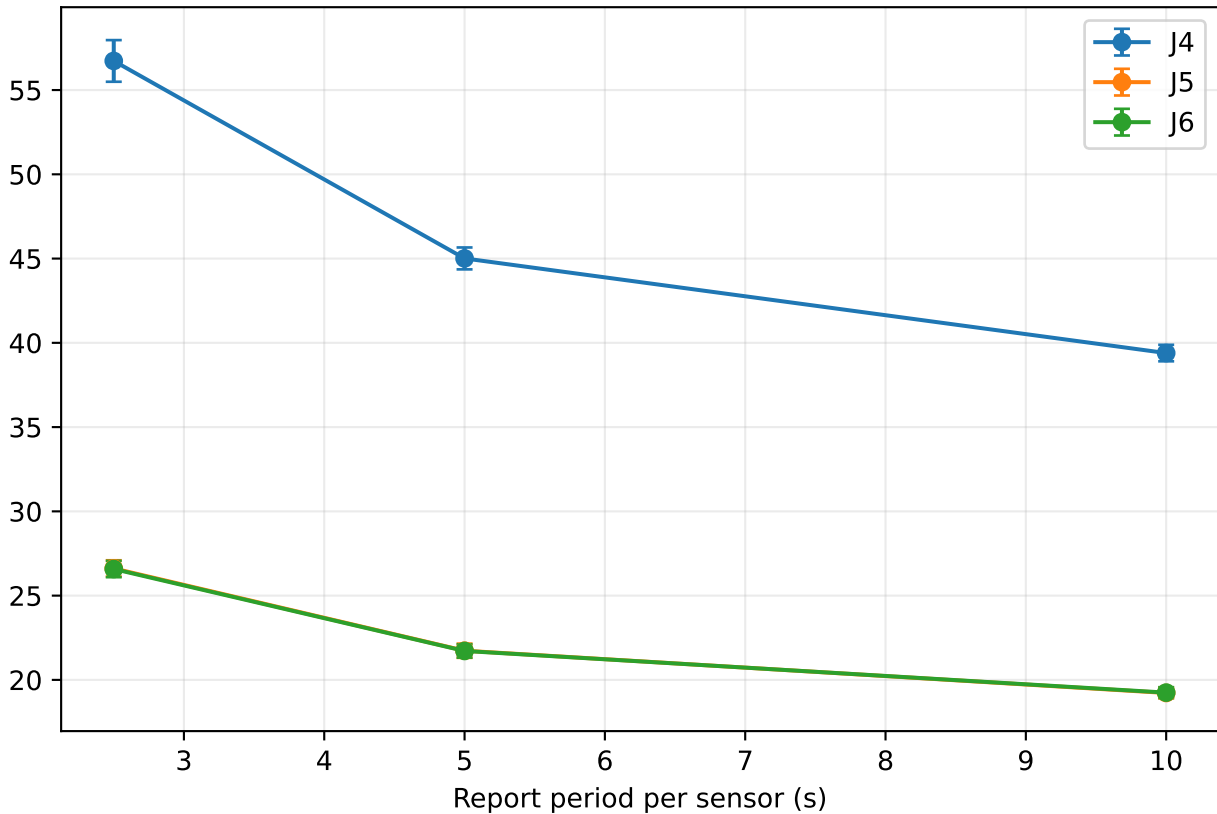
Delivered-report service delay (ms)
