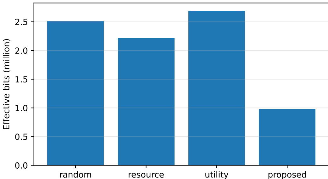
Intel Lab: Effective bits (million) at correlation 0.9
