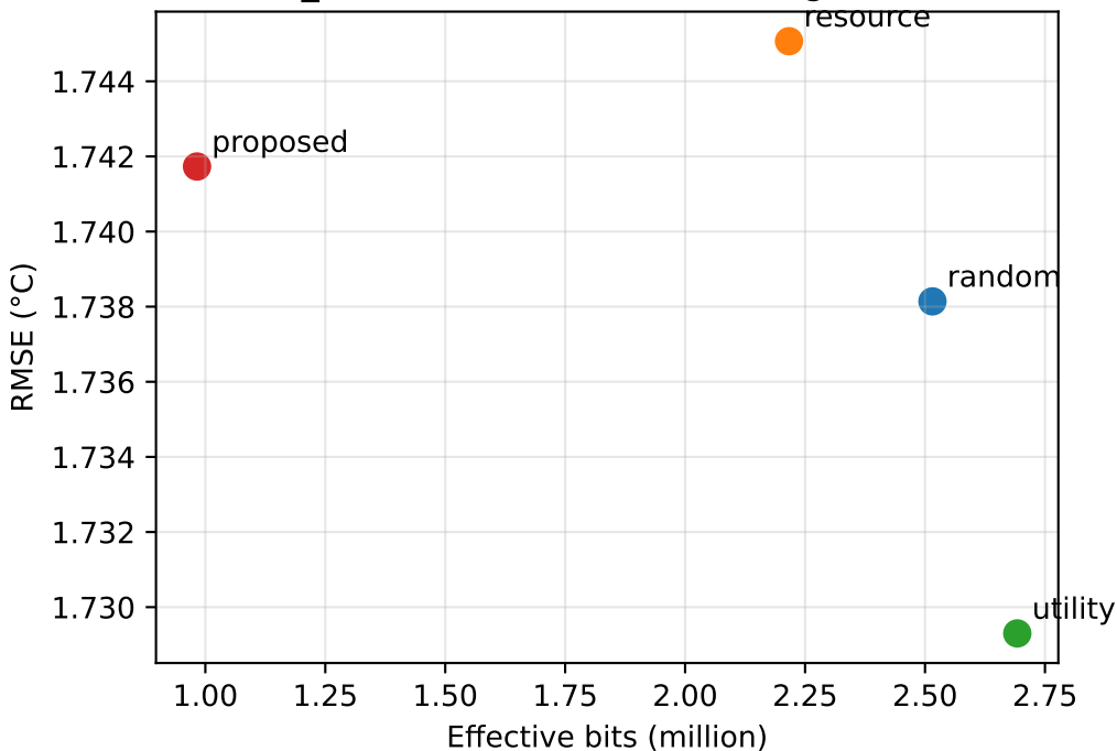
intel_lab: communication-learning trade-off
